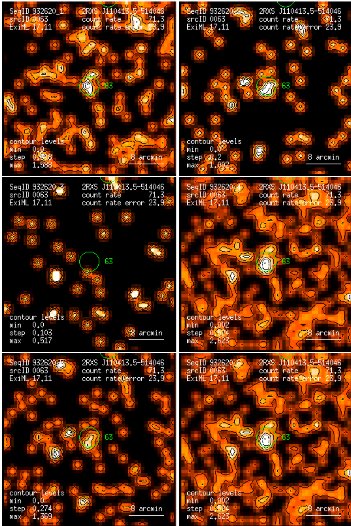
Figure 63: RASS 932620: detection 0063: band rate images, Gaussian filter: (1) PSPC channels 11 – 41, (2) 52 – 90, (3) 91 – 201, (4) 11 – 235, (5) 52 – 201, (6) 11 – 201. Broad band rates in counts/ks. Band rate contour levels in counts/ks/arcmin 2 .
