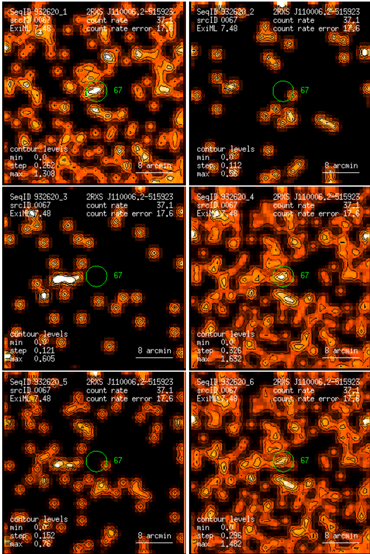
Figure 67: RASS 932620: detection 0067: band rate images, Gaussian filter: (1) PSPC channels 11 – 41, (2) 52 – 90, (3) 91 – 201, (4) 11 – 235, (5) 52 – 201, (6) 11 – 201. Broad band rates in counts/ks. Band rate contour levels in counts/ks/arcmin 2 .
