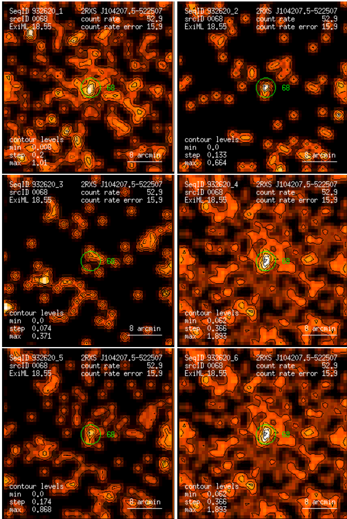
Figure 68: RASS 932620: detection 0068: band rate images, Gaussian filter: (1) PSPC channels 11 – 41, (2) 52 – 90, (3) 91 – 201, (4) 11 – 235, (5) 52 – 201, (6) 11 – 201. Broad band rates in counts/ks. Band rate contour levels in counts/ks/arcmin 2 .
