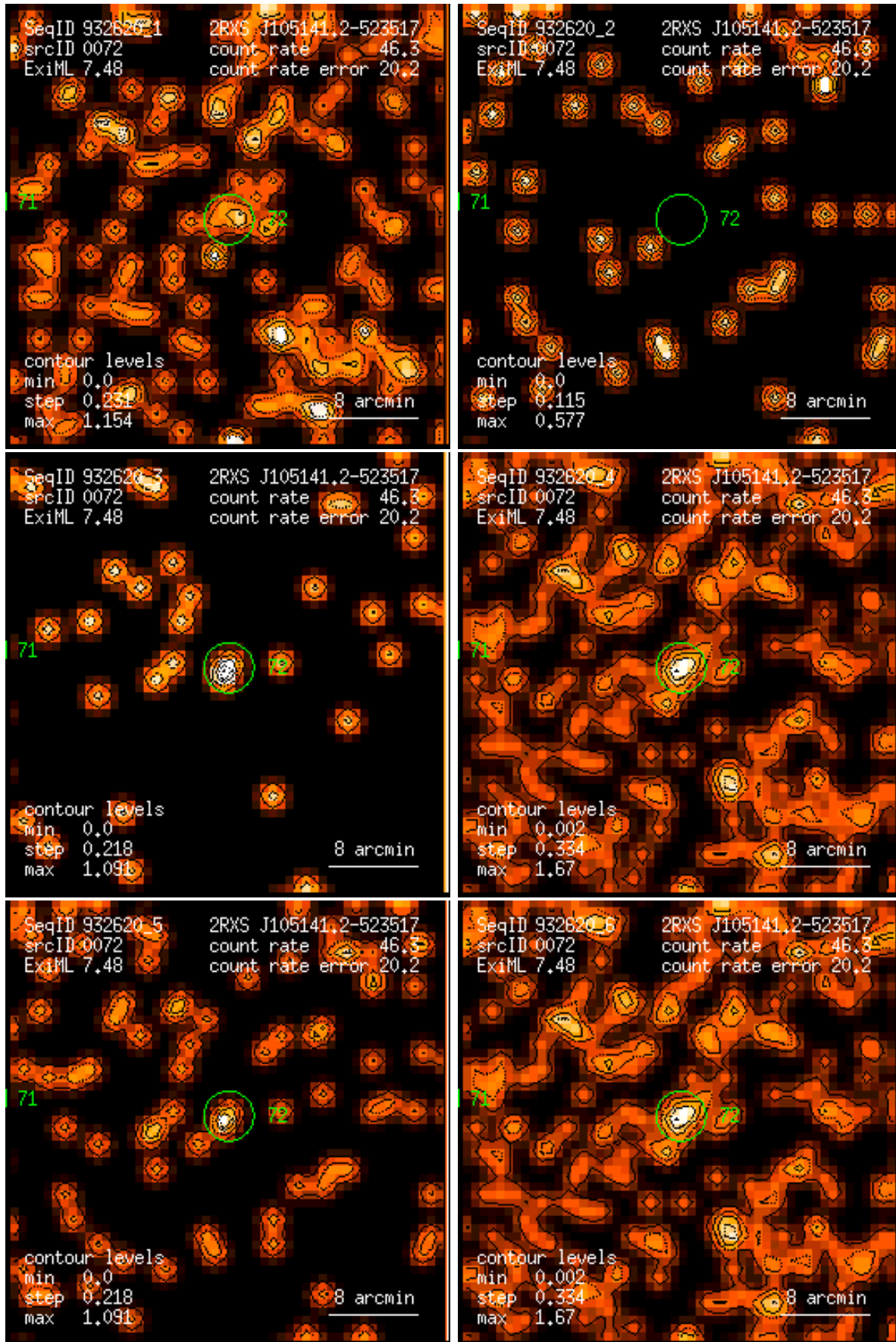
Figure 72: RASS 932620: detection 0072: band rate images, Gaussian filter: (1) PSPC channels 11 – 41, (2) 52 – 90, (3) 91 – 201, (4) 11 – 235, (5) 52 – 201, (6) 11 – 201. Broad band rates in counts/ks. Band rate contour levels in counts/ks/arcmin 2 .
