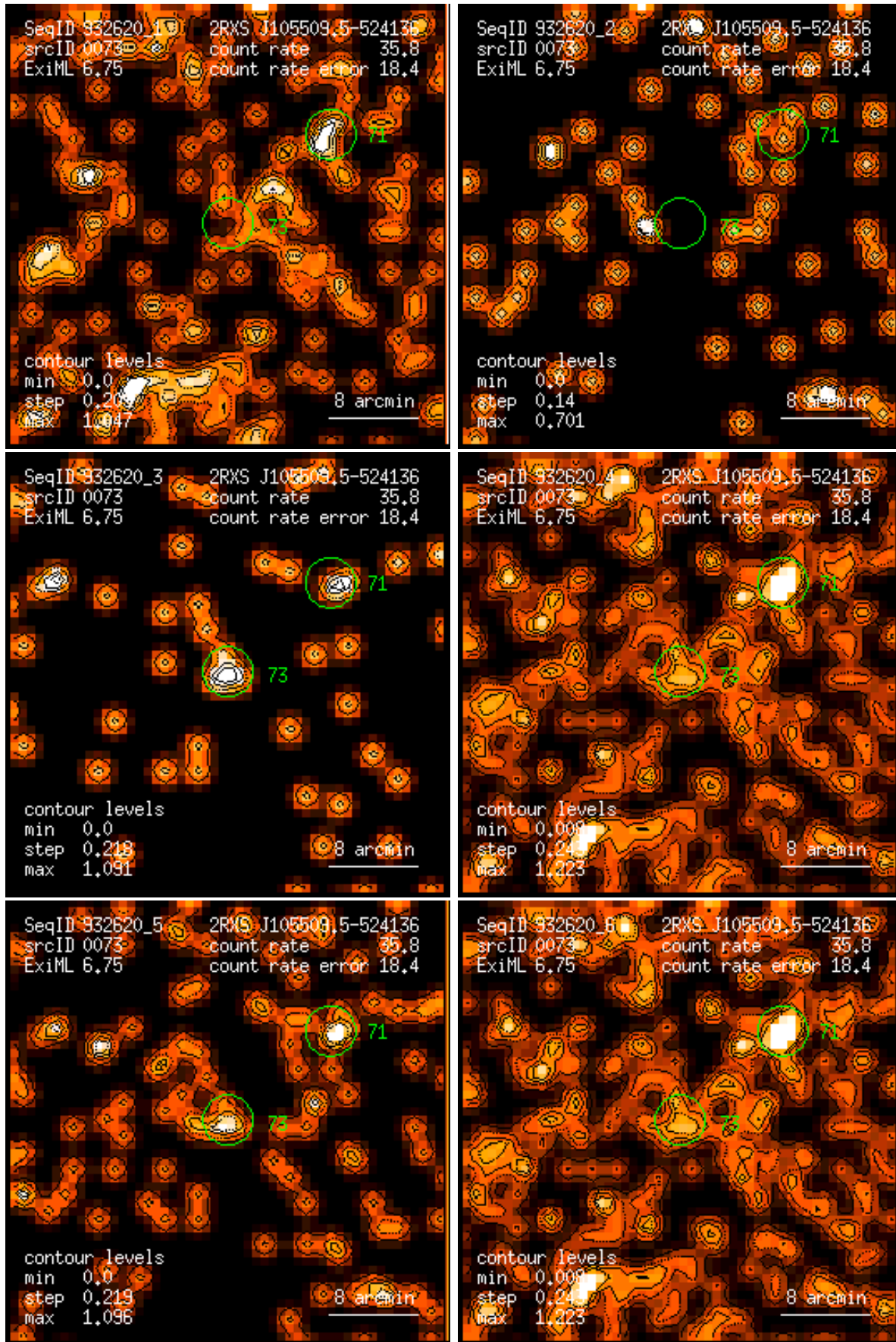
Figure 73: RASS 932620: detection 0073: band rate images, Gaussian filter: (1) PSPC channels 11 – 41, (2) 52 – 90, (3) 91 – 201, (4) 11 – 235, (5) 52 – 201, (6) 11 – 201. Broad band rates in counts/ks. Band rate contour levels in counts/ks/arcmin 2 .
