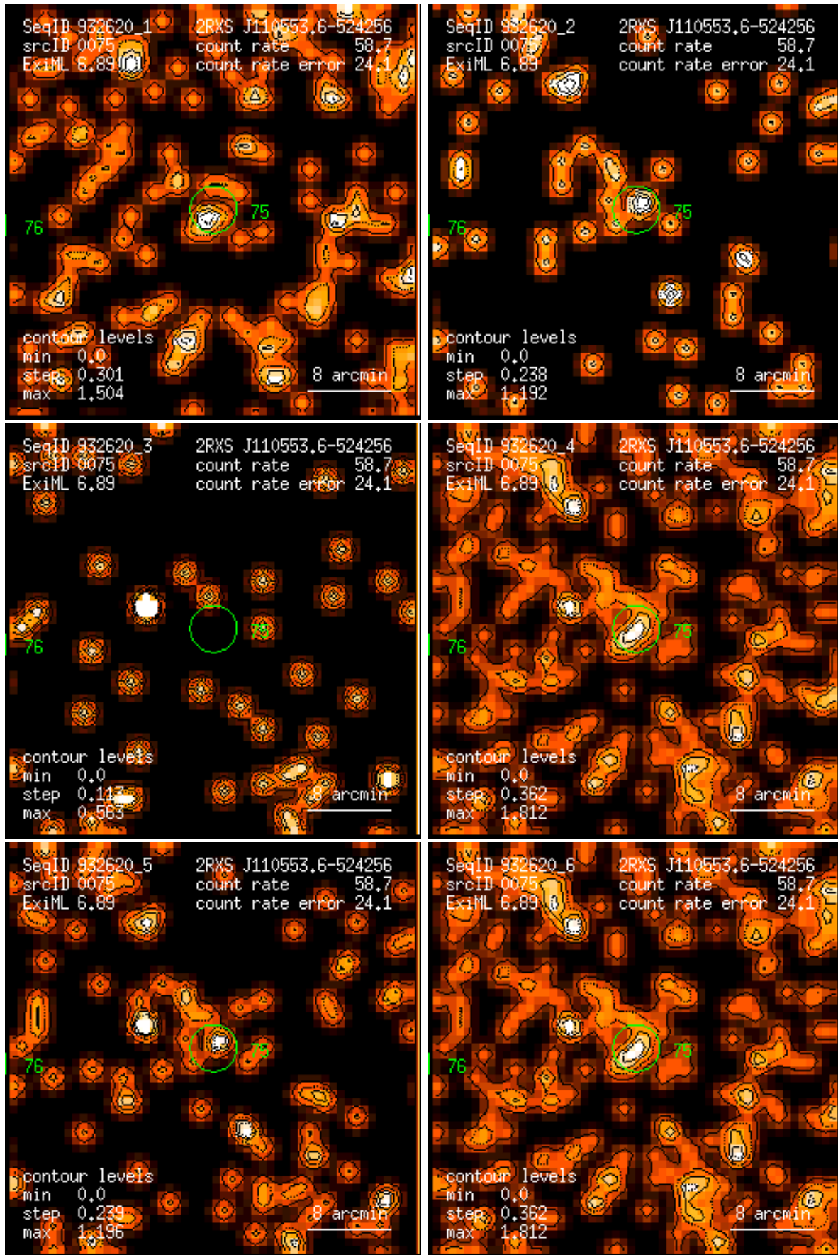
Figure 75: RASS 932620: detection 0075: band rate images, Gaussian filter: (1) PSPC channels 11 – 41, (2) 52 – 90, (3) 91 – 201, (4) 11 – 235, (5) 52 – 201, (6) 11 – 201. Broad band rates in counts/ks. Band rate contour levels in counts/ks/arcmin 2 .
