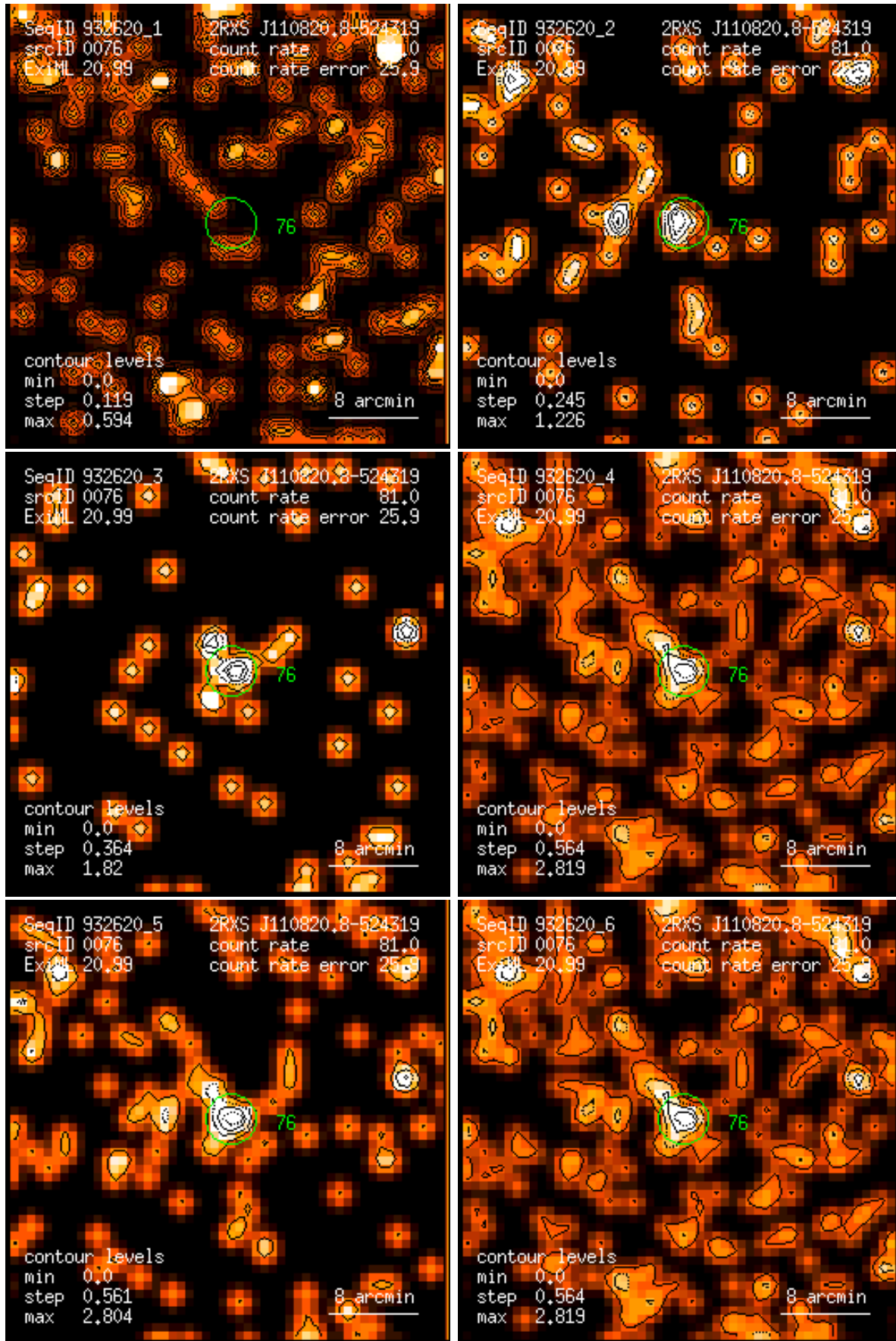
Figure 76: RASS 932620: detection 0076: band rate images, Gaussian filter: (1) PSPC channels 11 – 41, (2) 52 – 90, (3) 91 – 201, (4) 11 – 235, (5) 52 – 201, (6) 11 – 201. Broad band rates in counts/ks. Band rate contour levels in counts/ks/arcmin 2 .
