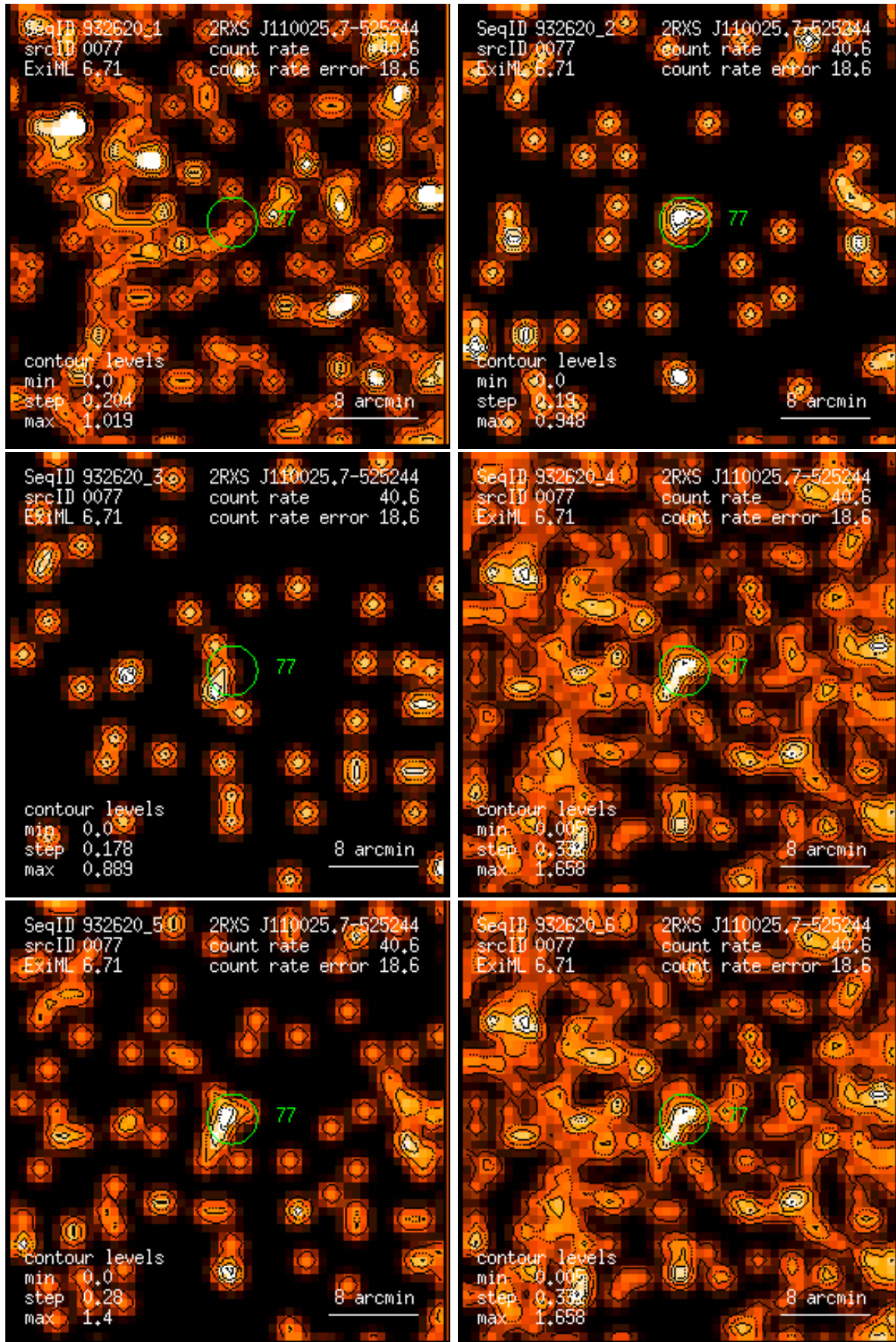
Figure 77: RASS 932620: detection 0077: band rate images, Gaussian filter: (1) PSPC channels 11 – 41, (2) 52 – 90, (3) 91 – 201, (4) 11 – 235, (5) 52 – 201, (6) 11 – 201. Broad band rates in counts/ks. Band rate contour levels in counts/ks/arcmin 2 .
