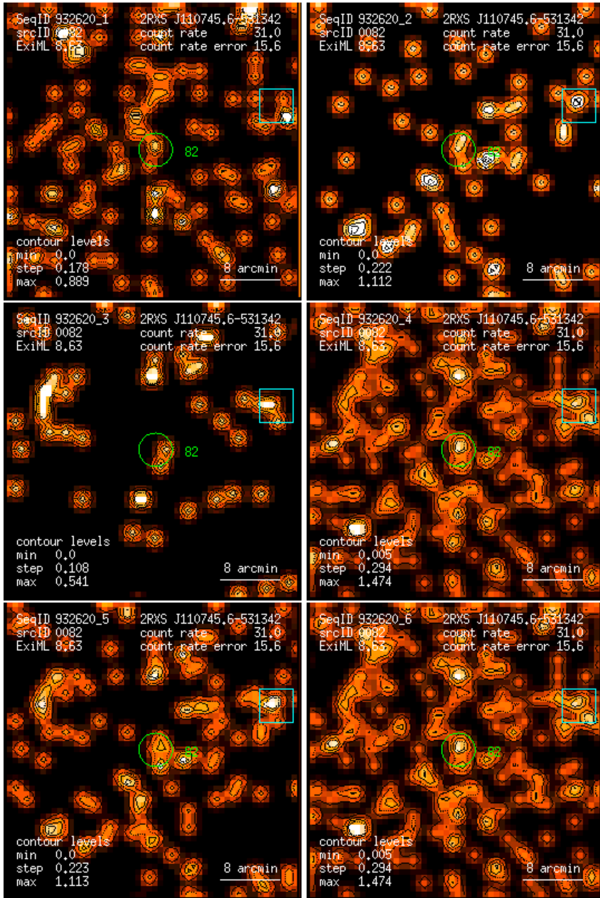
Figure 82: RASS 932620: detection 0082: band rate images, Gaussian filter: (1) PSPC channels 11 – 41, (2) 52 – 90, (3) 91 – 201, (4) 11 – 235, (5) 52 – 201, (6) 11 – 201. Broad band rates in counts/ks. Band rate contour levels in counts/ks/arcmin 2 .
