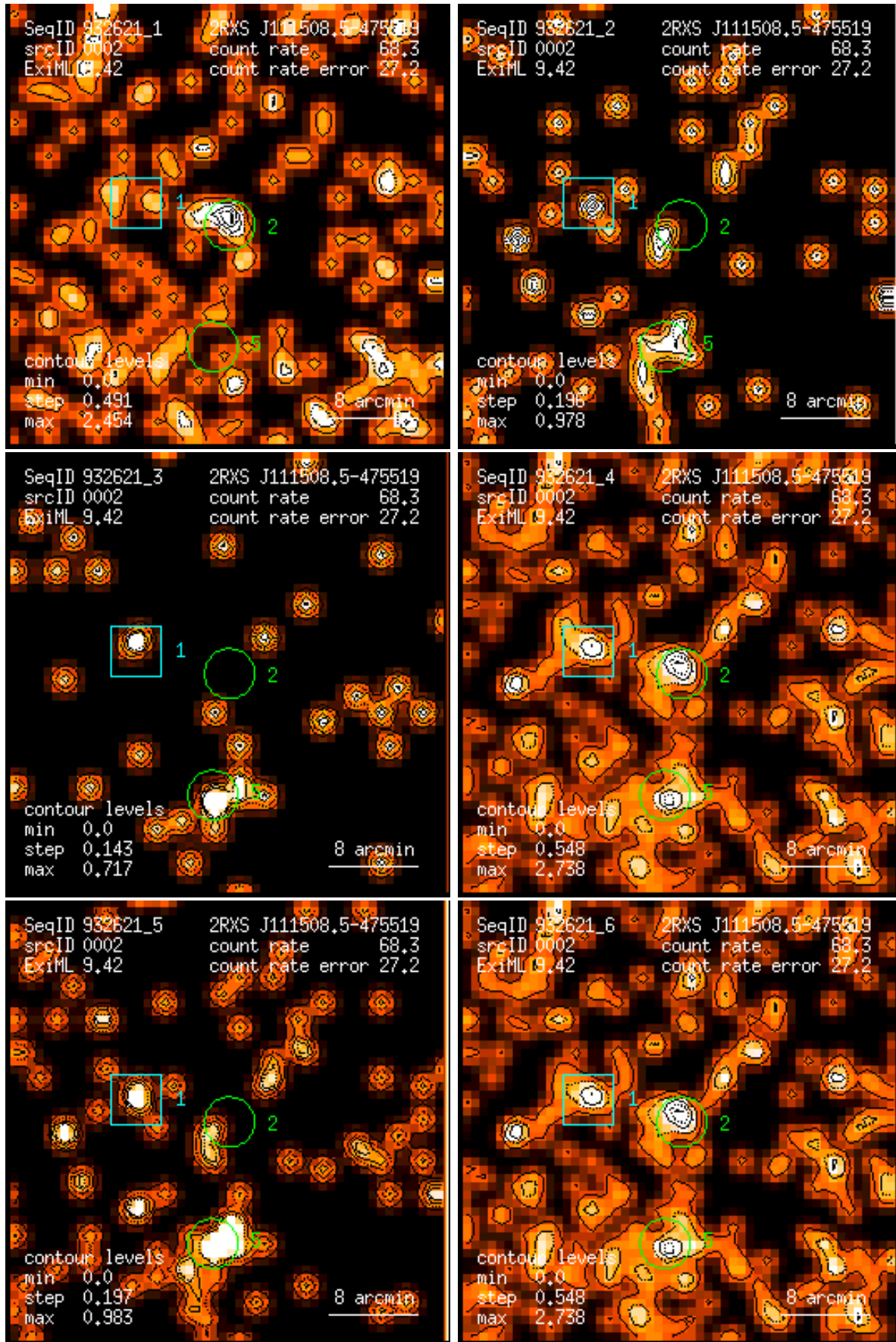
Figure 2: RASS 932621: detection 0002: band rate images, Gaussian filter: (1) PSPC channels 11 – 41, (2) 52 – 90, (3) 91 – 201, (4) 11 – 235, (5) 52 – 201, (6) 11 – 201. Broad band rates in counts/ks. Band rate contour levels in counts/ks/arcmin 2 .
