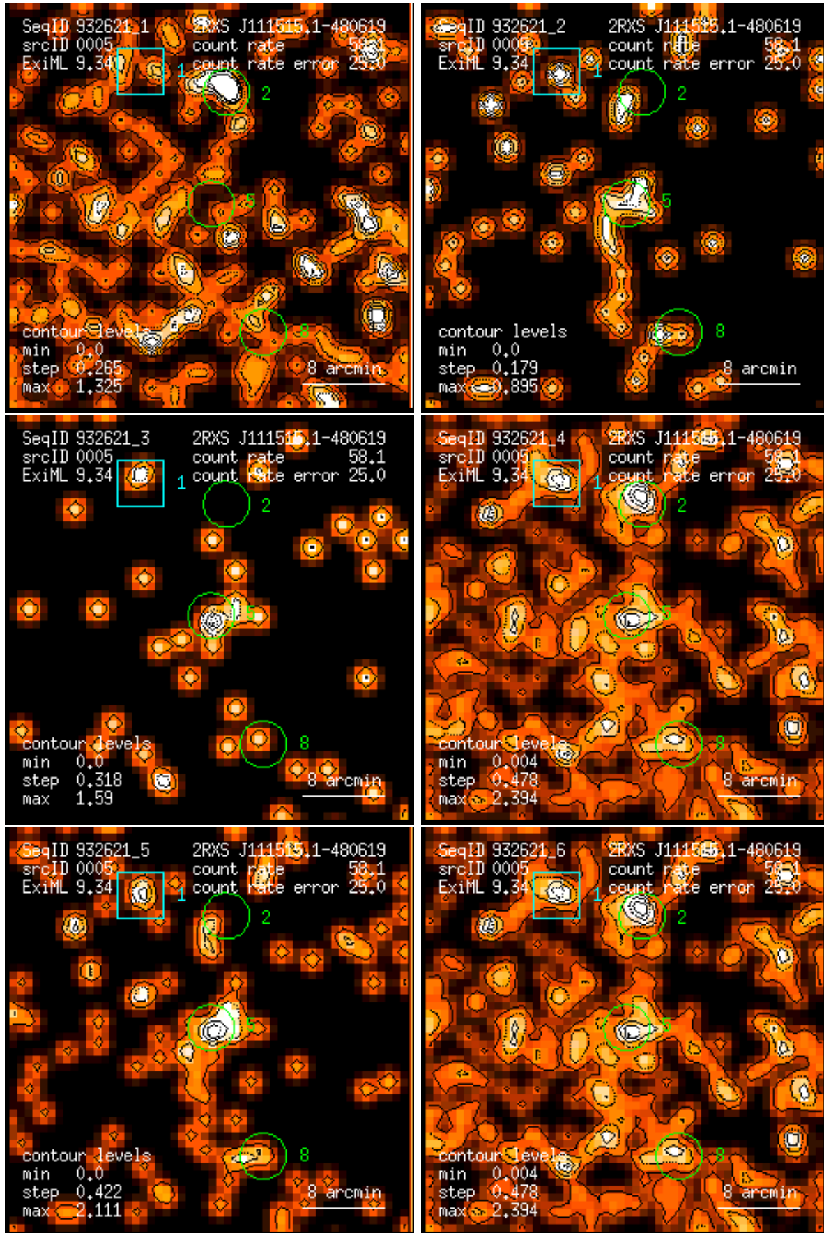
Figure 5: RASS 932621: detection 0005: band rate images, Gaussian filter: (1) PSPC channels 11 – 41, (2) 52 – 90, (3) 91 – 201, (4) 11 – 235, (5) 52 – 201, (6) 11 – 201. Broad band rates in counts/ks. Band rate contour levels in counts/ks/arcmin 2 .
