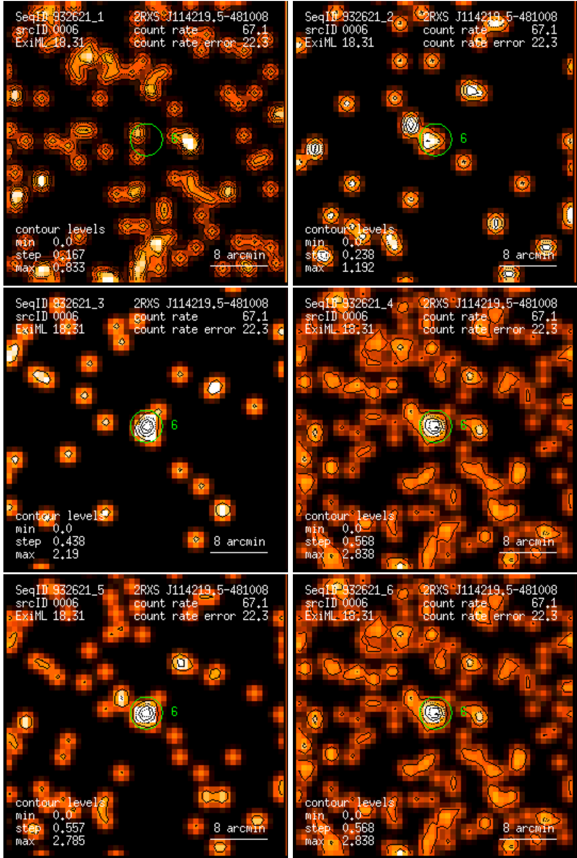
Figure 6: RASS 932621: detection 0006: band rate images, Gaussian filter: (1) PSPC channels 11 – 41, (2) 52 – 90, (3) 91 – 201, (4) 11 – 235, (5) 52 – 201, (6) 11 – 201. Broad band rates in counts/ks. Band rate contour levels in counts/ks/arcmin 2 .
