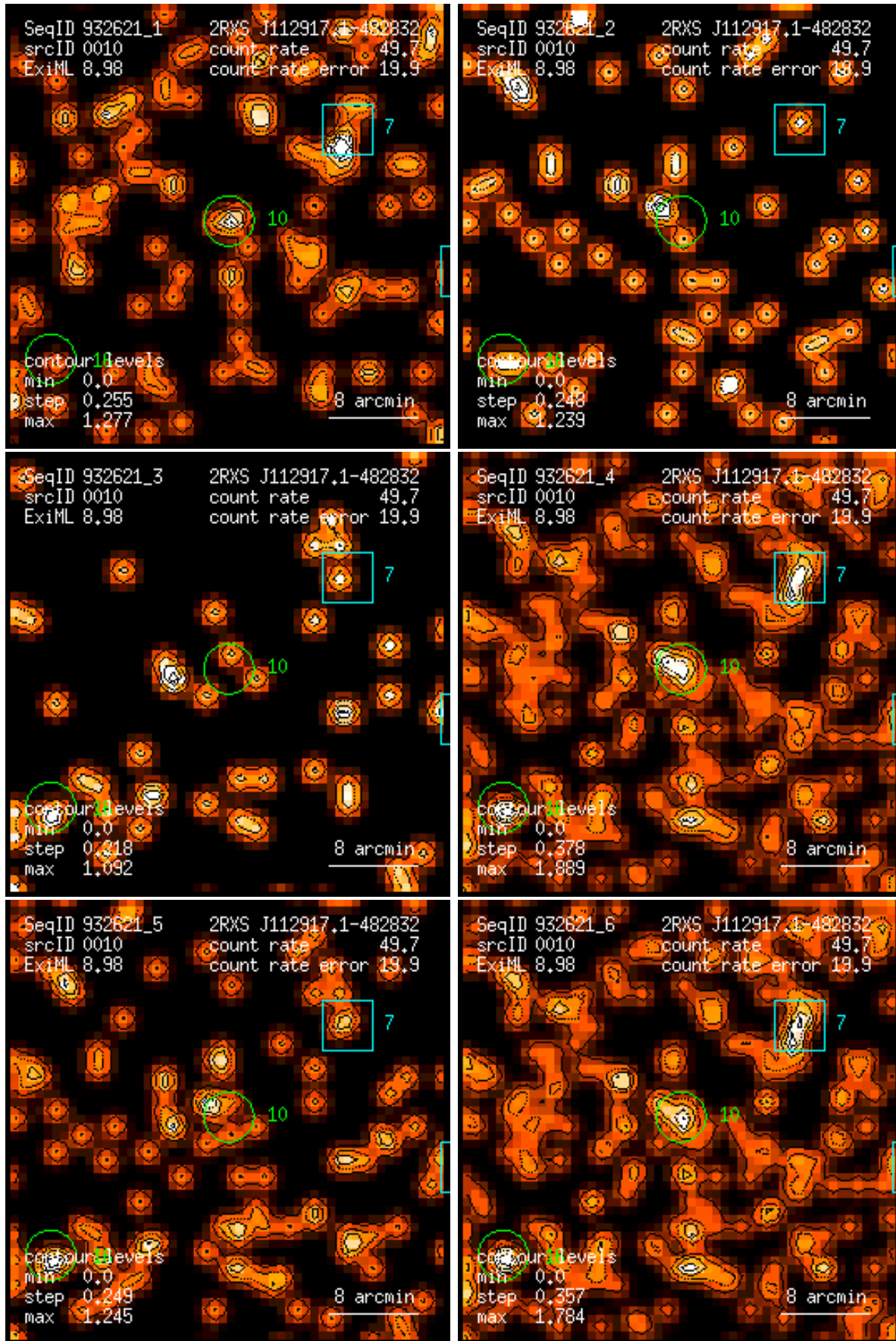
Figure 10: RASS 932621: detection 0010: band rate images, Gaussian filter: (1) PSPC channels 11 – 41, (2) 52 – 90, (3) 91 – 201, (4) 11 – 235, (5) 52 – 201, (6) 11 – 201. Broad band rates in counts/ks. Band rate contour levels in counts/ks/arcmin 2 .
