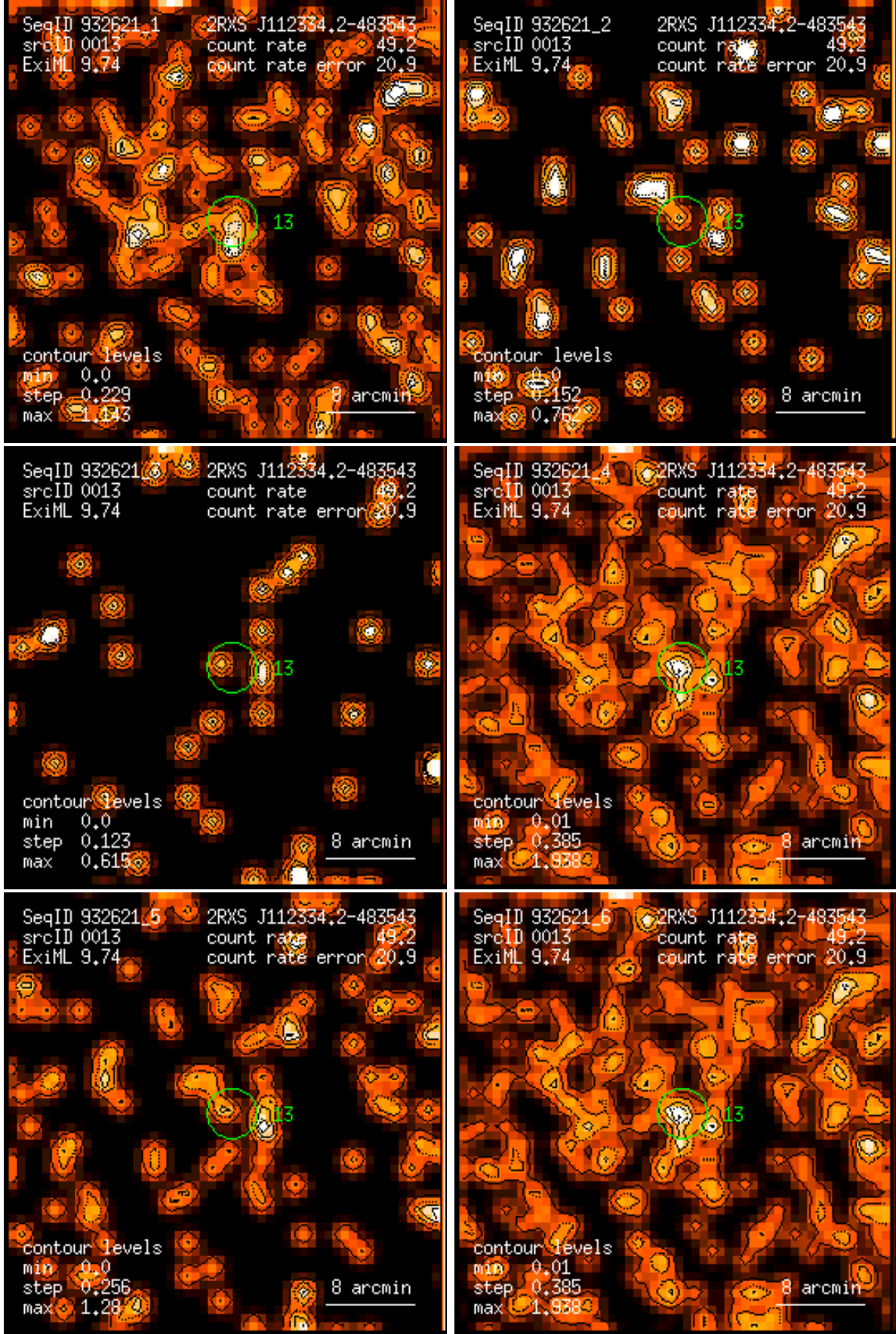
Figure 13: RASS 932621: detection 0013: band rate images, Gaussian filter: (1) PSPC channels 11 – 41, (2) 52 – 90, (3) 91 – 201, (4) 11 – 235, (5) 52 – 201, (6) 11 – 201. Broad band rates in counts/ks. Band rate contour levels in counts/ks/arcmin 2 .
