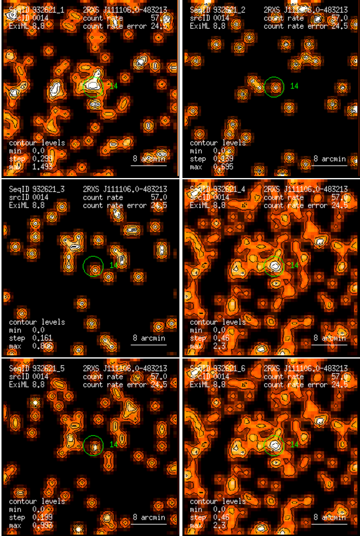
Figure 14: RASS 932621: detection 0014: band rate images, Gaussian filter: (1) PSPC channels 11 – 41, (2) 52 – 90, (3) 91 – 201, (4) 11 – 235, (5) 52 – 201, (6) 11 – 201. Broad band rates in counts/ks. Band rate contour levels in counts/ks/arcmin 2 .
