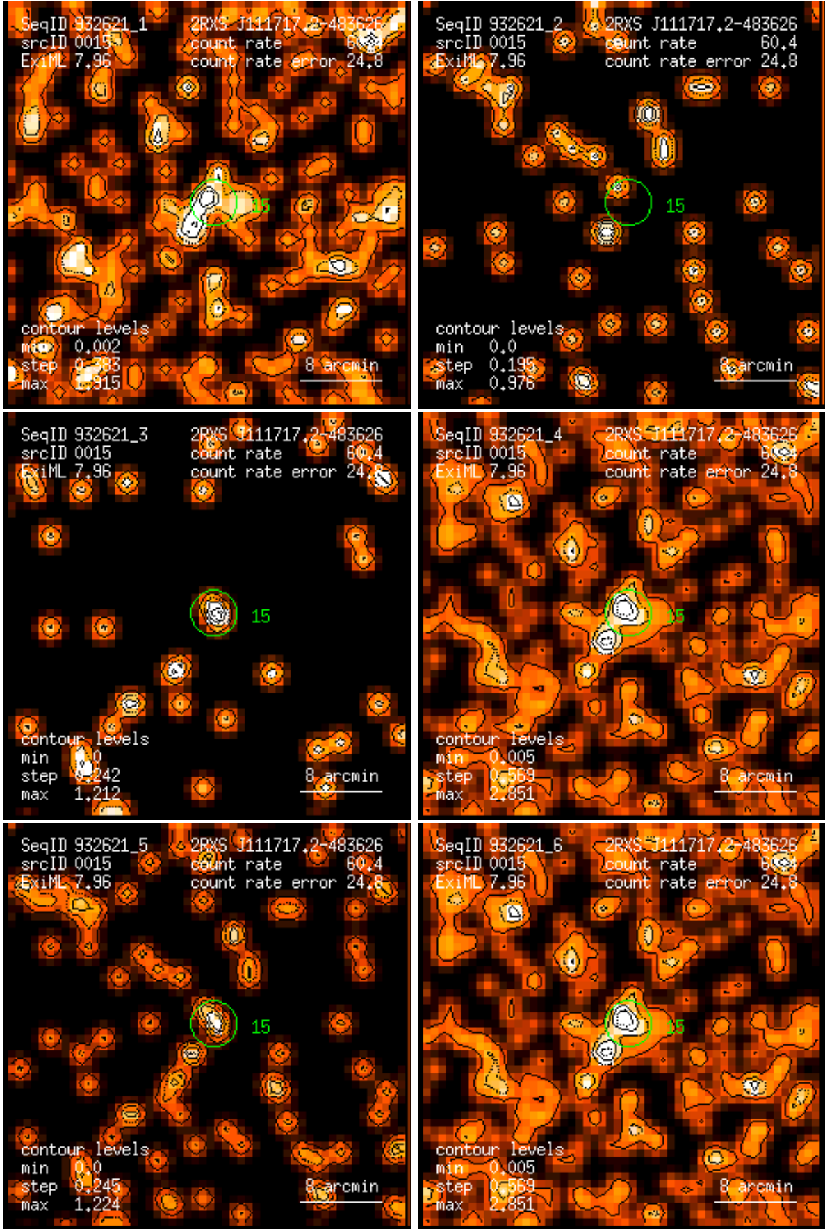
Figure 15: RASS 932621: detection 0015: band rate images, Gaussian filter: (1) PSPC channels 11 – 41, (2) 52 – 90, (3) 91 – 201, (4) 11 – 235, (5) 52 – 201, (6) 11 – 201. Broad band rates in counts/ks. Band rate contour levels in counts/ks/arcmin 2 .
