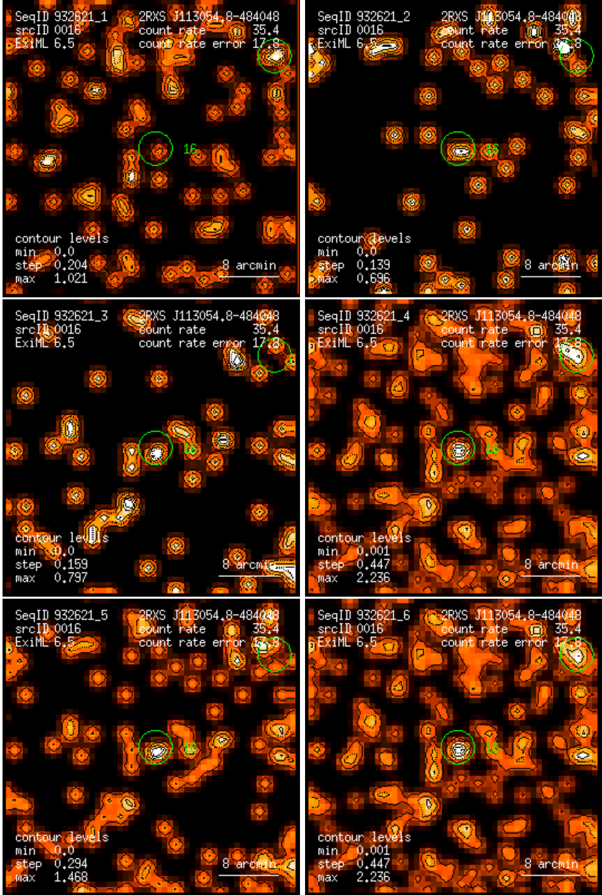
Figure 16: RASS 932621: detection 0016: band rate images, Gaussian filter: (1) PSPC channels 11 – 41, (2) 52 – 90, (3) 91 – 201, (4) 11 – 235, (5) 52 – 201, (6) 11 – 201. Broad band rates in counts/ks. Band rate contour levels in counts/ks/arcmin 2 .
