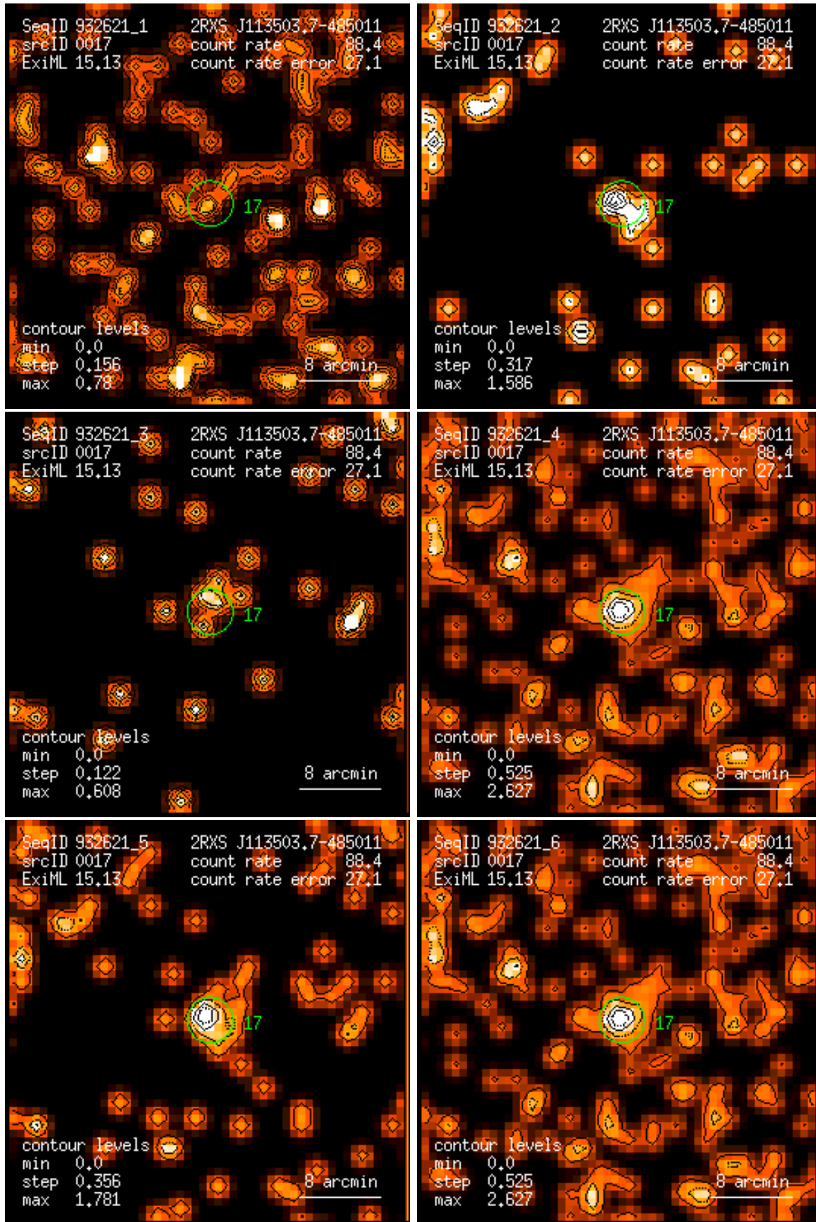
Figure 17: RASS 932621: detection 0017: band rate images, Gaussian filter: (1) PSPC channels 11 – 41, (2) 52 – 90, (3) 91 – 201, (4) 11 – 235, (5) 52 – 201, (6) 11 – 201. Broad band rates in counts/ks. Band rate contour levels in counts/ks/arcmin 2 .
