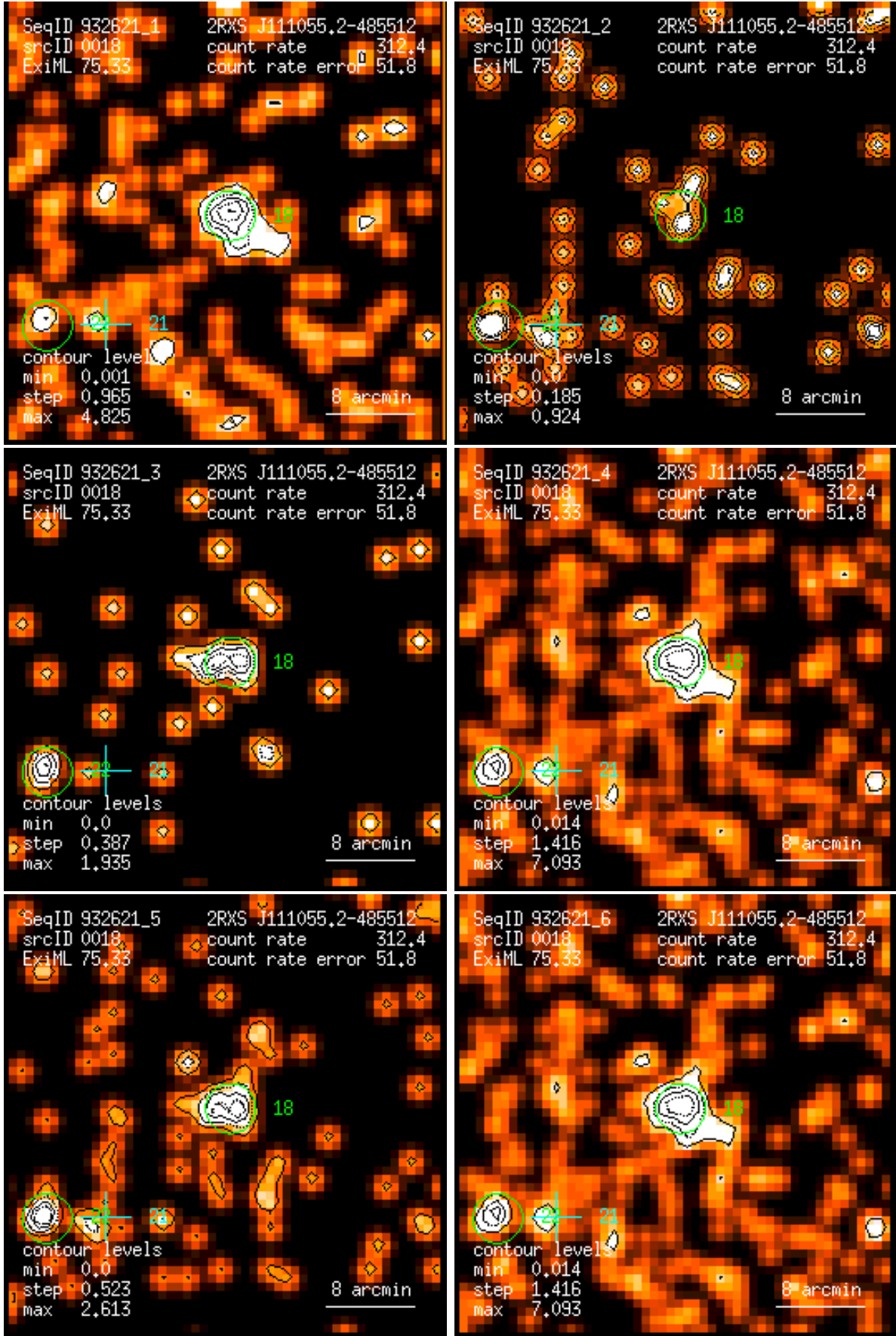
Figure 18: RASS 932621: detection 0018: band rate images, Gaussian filter: (1) PSPC channels 11 – 41, (2) 52 – 90, (3) 91 – 201, (4) 11 – 235, (5) 52 – 201, (6) 11 – 201. Broad band rates in counts/ks. Band rate contour levels in counts/ks/arcmin 2 .
