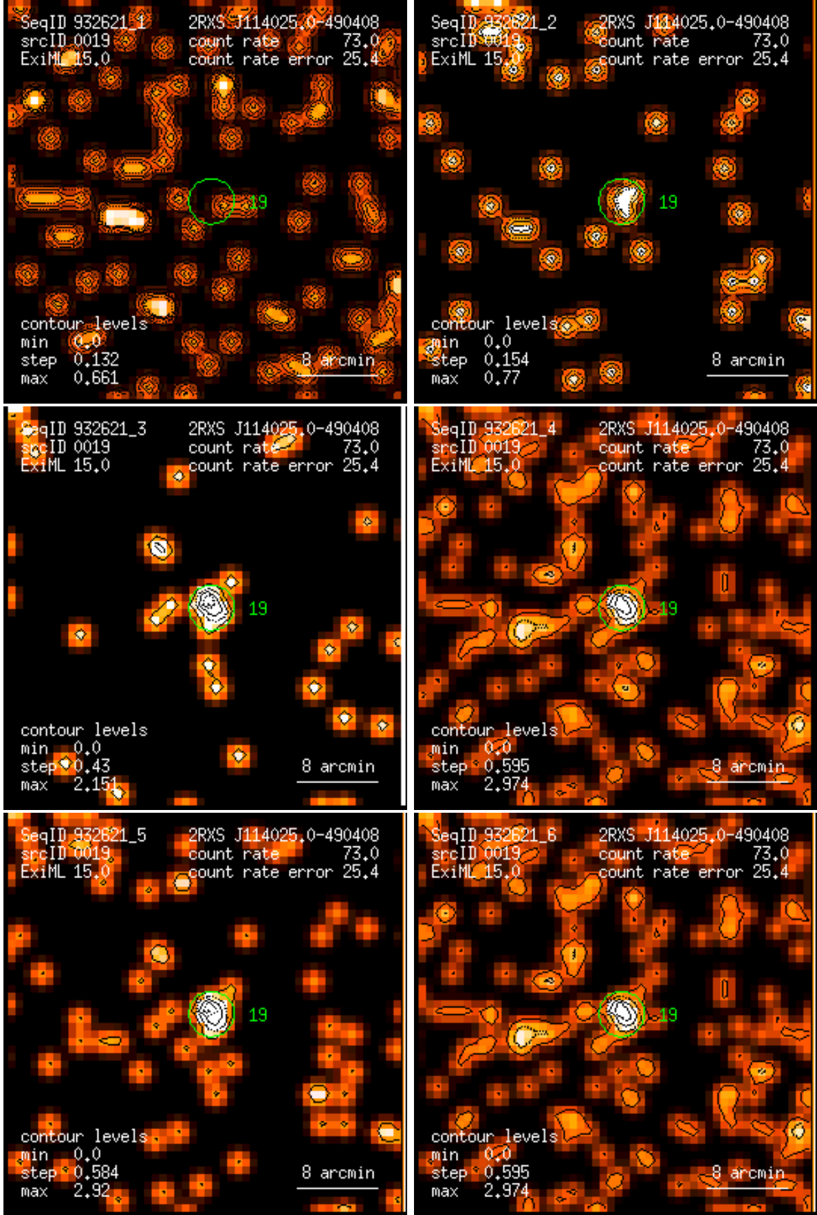
Figure 19: RASS 932621: detection 0019: band rate images, Gaussian filter: (1) PSPC channels 11 – 41, (2) 52 – 90, (3) 91 – 201, (4) 11 – 235, (5) 52 – 201, (6) 11 – 201. Broad band rates in counts/ks. Band rate contour levels in counts/ks/arcmin 2 .
