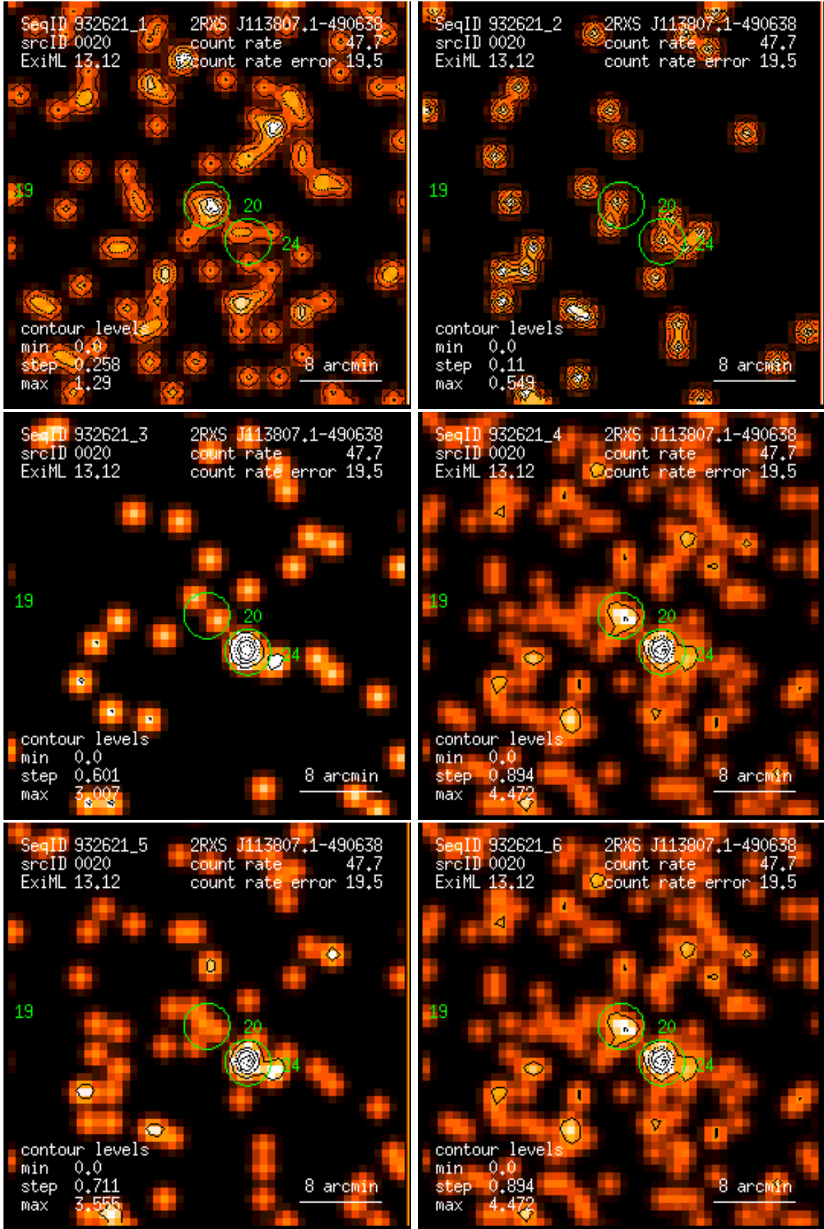
Figure 20: RASS 932621: detection 0020: band rate images, Gaussian filter: (1) PSPC channels 11 – 41, (2) 52 – 90, (3) 91 – 201, (4) 11 – 235, (5) 52 – 201, (6) 11 – 201. Broad band rates in counts/ks. Band rate contour levels in counts/ks/arcmin 2 .
