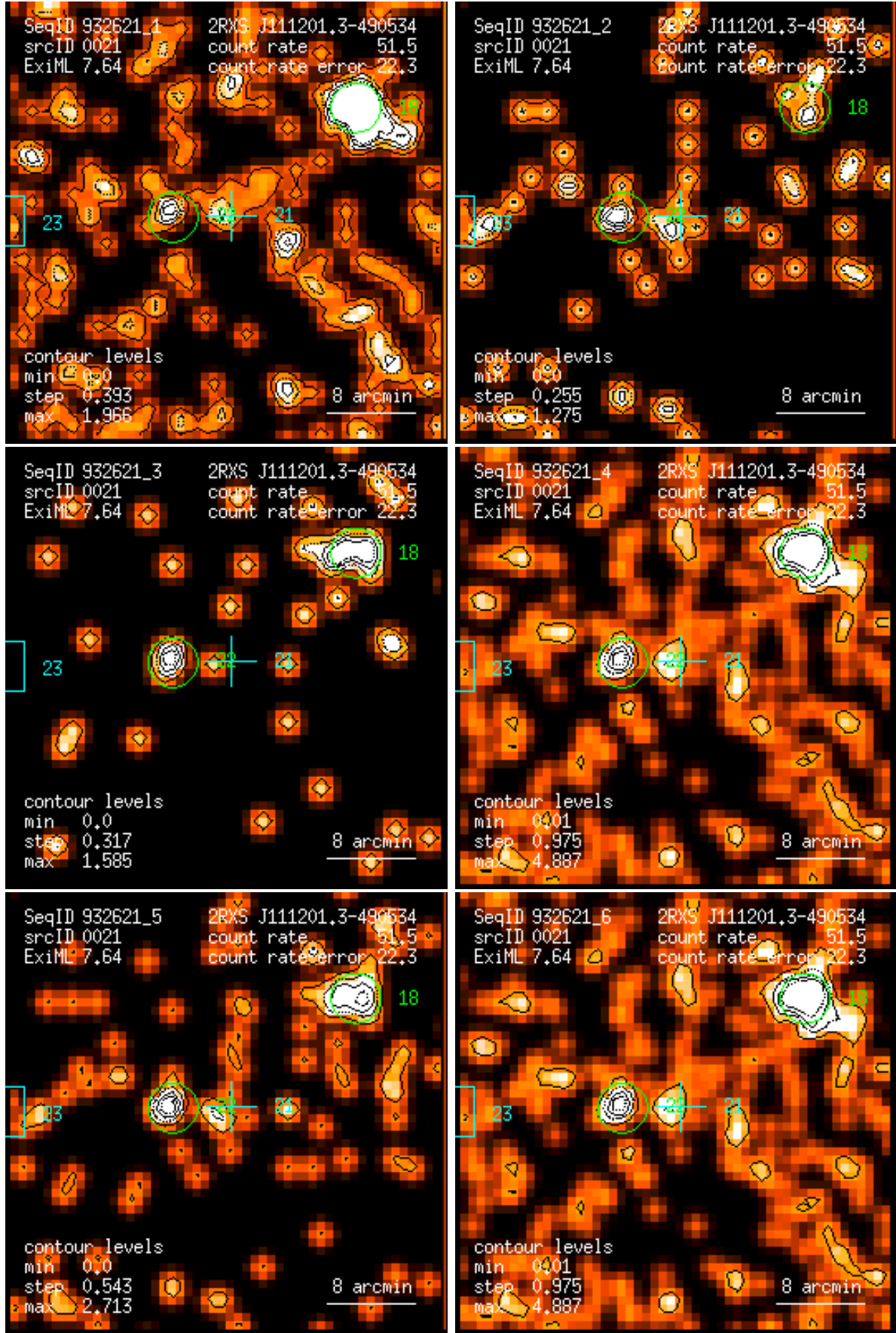
Figure 21: RASS 932621: detection 0021: band rate images, Gaussian filter: (1) PSPC channels 11 – 41, (2) 52 – 90, (3) 91 – 201, (4) 11 – 235, (5) 52 – 201, (6) 11 – 201. Broad band rates in counts/ks. Band rate contour levels in counts/ks/arcmin 2 .
