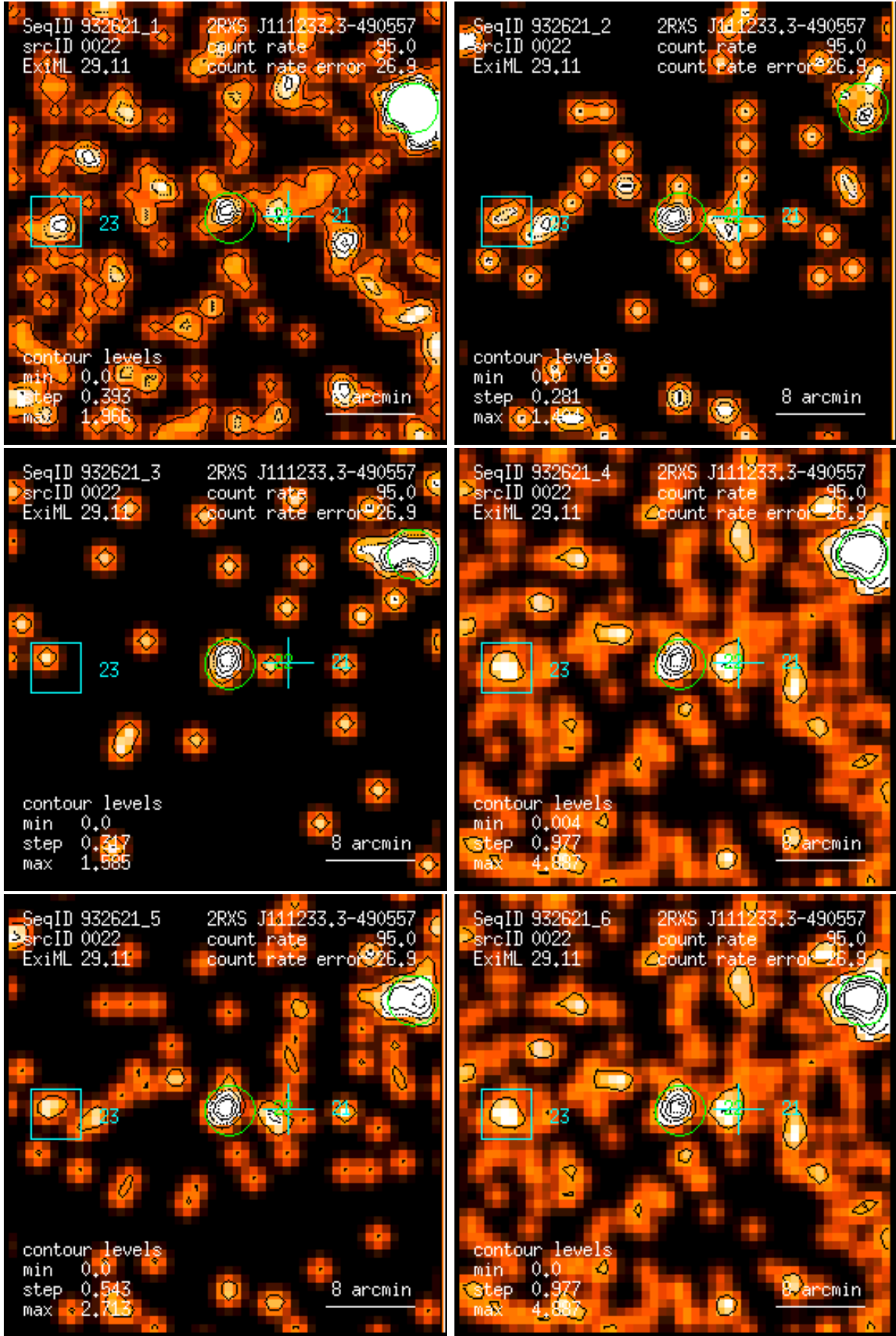
Figure 22: RASS 932621: detection 0022: band rate images, Gaussian filter: (1) PSPC channels 11 – 41, (2) 52 – 90, (3) 91 – 201, (4) 11 – 235, (5) 52 – 201, (6) 11 – 201. Broad band rates in counts/ks. Band rate contour levels in counts/ks/arcmin 2 .
