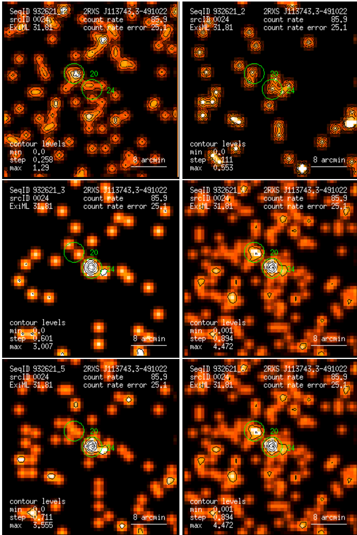
Figure 24: RASS 932621: detection 0024: band rate images, Gaussian filter: (1) PSPC channels 11 – 41, (2) 52 – 90, (3) 91 – 201, (4) 11 – 235, (5) 52 – 201, (6) 11 – 201. Broad band rates in counts/ks. Band rate contour levels in counts/ks/arcmin 2 .
