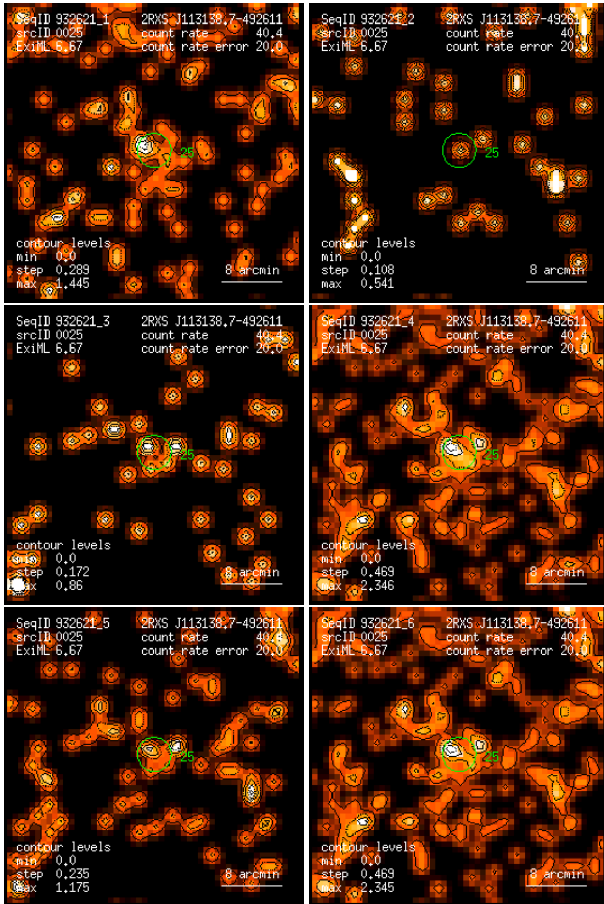
Figure 25: RASS 932621: detection 0025: band rate images, Gaussian filter: (1) PSPC channels 11 – 41, (2) 52 – 90, (3) 91 – 201, (4) 11 – 235, (5) 52 – 201, (6) 11 – 201. Broad band rates in counts/ks. Band rate contour levels in counts/ks/arcmin 2 .
