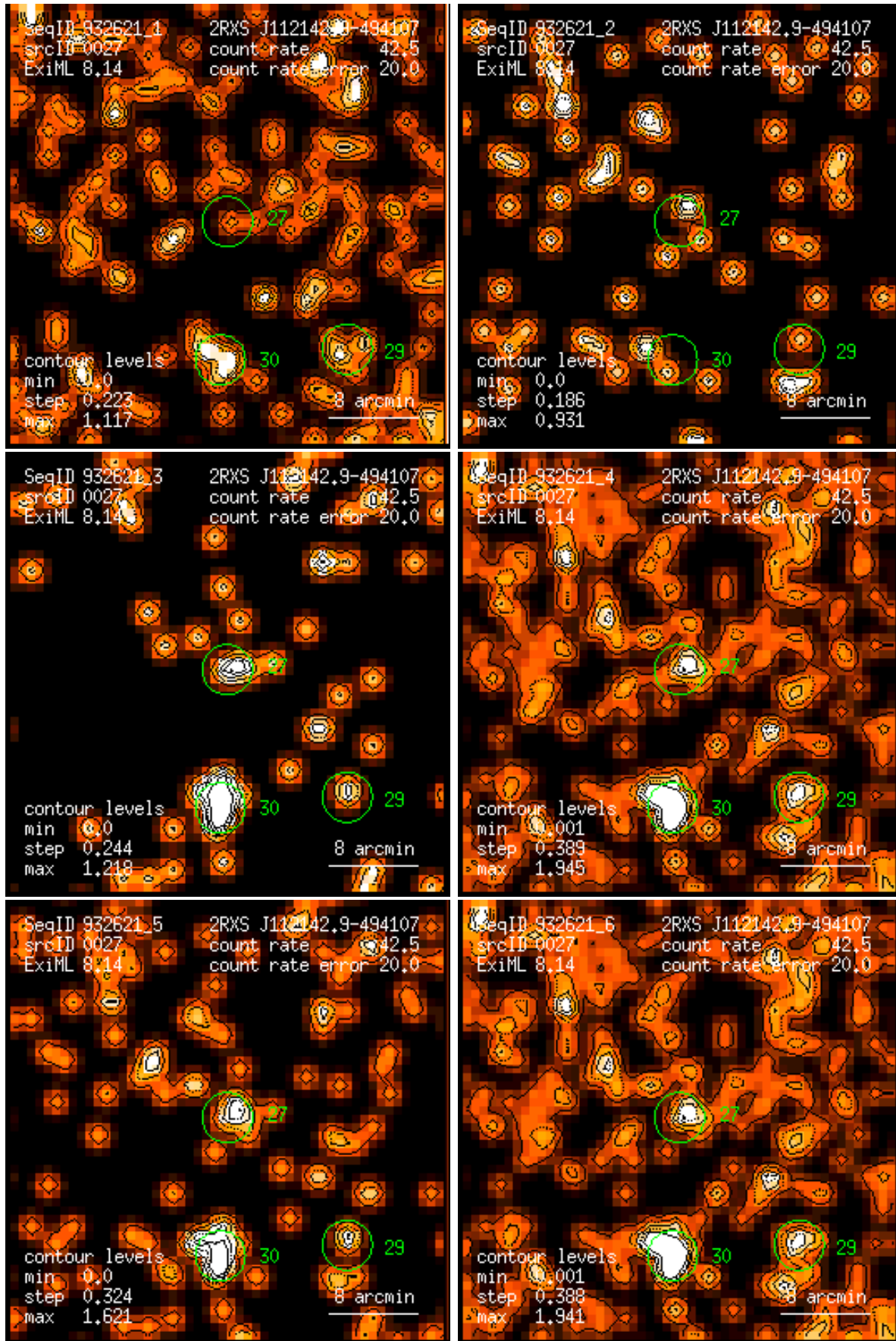
Figure 27: RASS 932621: detection 0027: band rate images, Gaussian filter: (1) PSPC channels 11 – 41, (2) 52 – 90, (3) 91 – 201, (4) 11 – 235, (5) 52 – 201, (6) 11 – 201. Broad band rates in counts/ks. Band rate contour levels in counts/ks/arcmin 2 .
