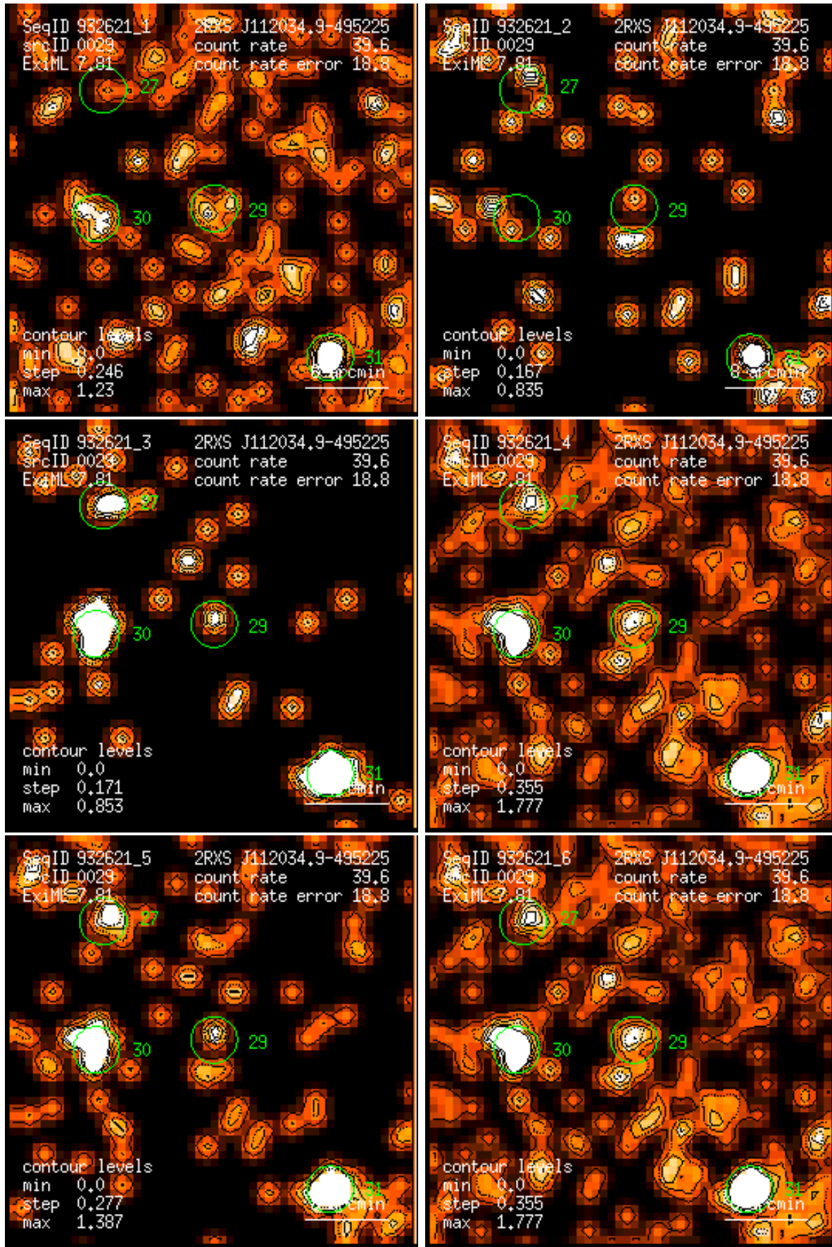
Figure 29: RASS 932621: detection 0029: band rate images, Gaussian filter: (1) PSPC channels 11 – 41, (2) 52 – 90, (3) 91 – 201, (4) 11 – 235, (5) 52 – 201, (6) 11 – 201. Broad band rates in counts/ks. Band rate contour levels in counts/ks/arcmin 2 .
