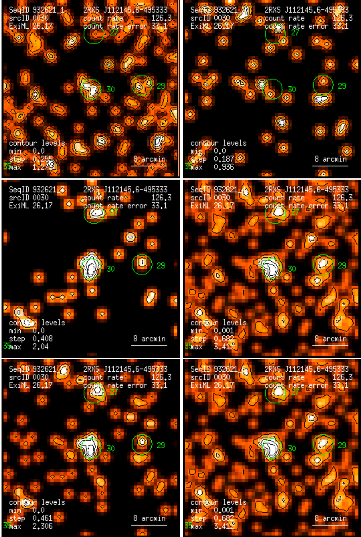
Figure 30: RASS 932621: detection 0030: band rate images, Gaussian filter: (1) PSPC channels 11 – 41, (2) 52 – 90, (3) 91 – 201, (4) 11 – 235, (5) 52 – 201, (6) 11 – 201. Broad band rates in counts/ks. Band rate contour levels in counts/ks/arcmin 2 .
