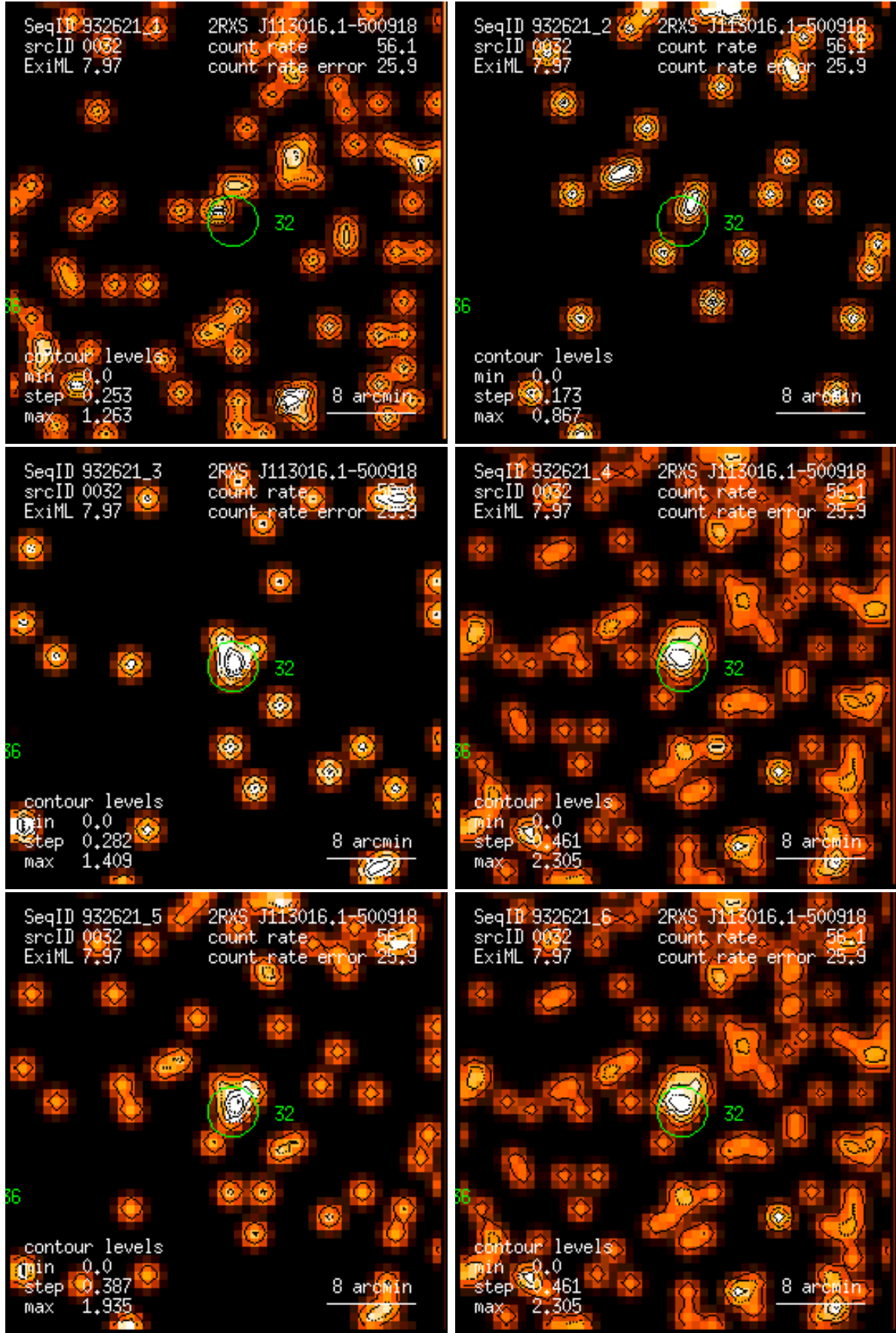
Figure 32: RASS 932621: detection 0032: band rate images, Gaussian filter: (1) PSPC channels 11 – 41, (2) 52 – 90, (3) 91 – 201, (4) 11 – 235, (5) 52 – 201, (6) 11 – 201. Broad band rates in counts/ks. Band rate contour levels in counts/ks/arcmin 2 .
