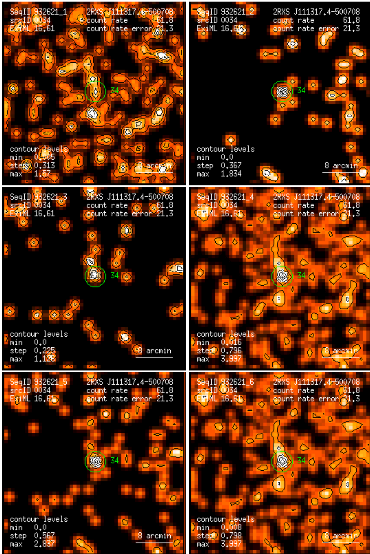
Figure 34: RASS 932621: detection 0034: band rate images, Gaussian filter: (1) PSPC channels 11 – 41, (2) 52 – 90, (3) 91 – 201, (4) 11 – 235, (5) 52 – 201, (6) 11 – 201. Broad band rates in counts/ks. Band rate contour levels in counts/ks/arcmin 2 .
