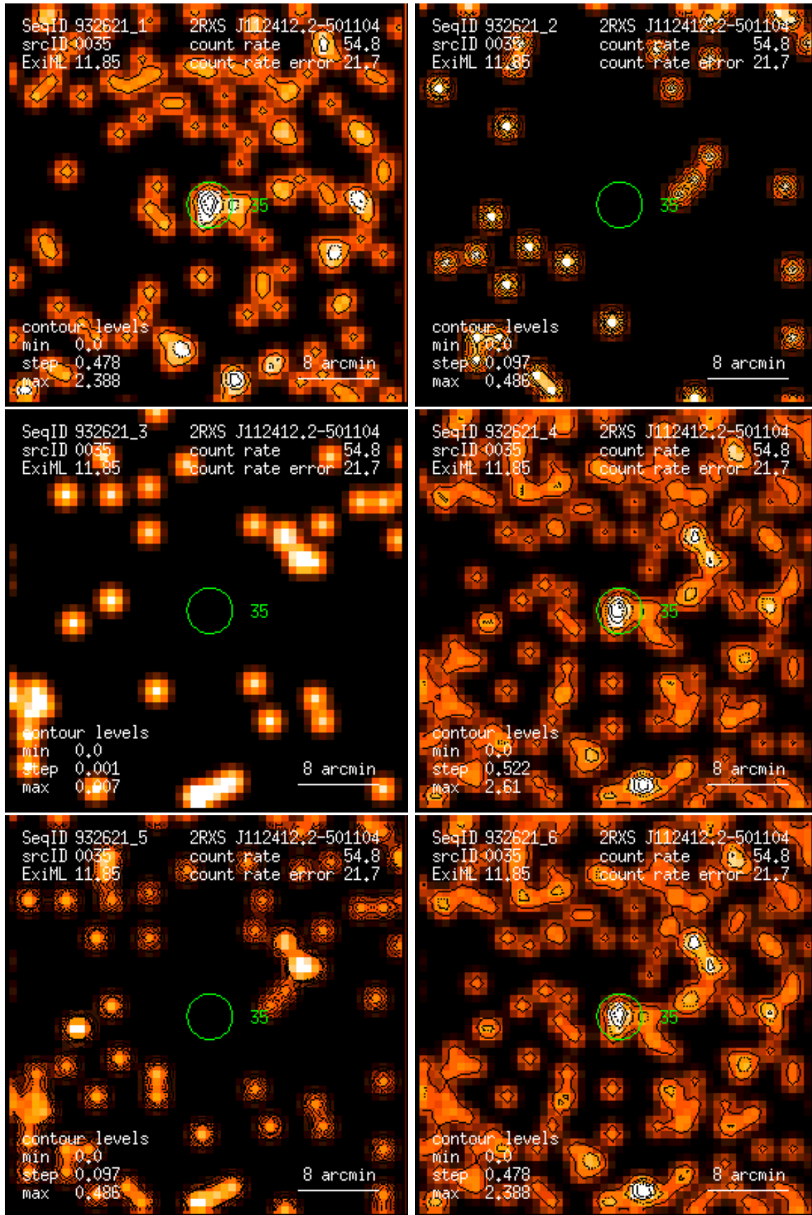
Figure 35: RASS 932621: detection 0035: band rate images, Gaussian filter: (1) PSPC channels 11 – 41, (2) 52 – 90, (3) 91 – 201, (4) 11 – 235, (5) 52 – 201, (6) 11 – 201. Broad band rates in counts/ks. Band rate contour levels in counts/ks/arcmin 2 .
