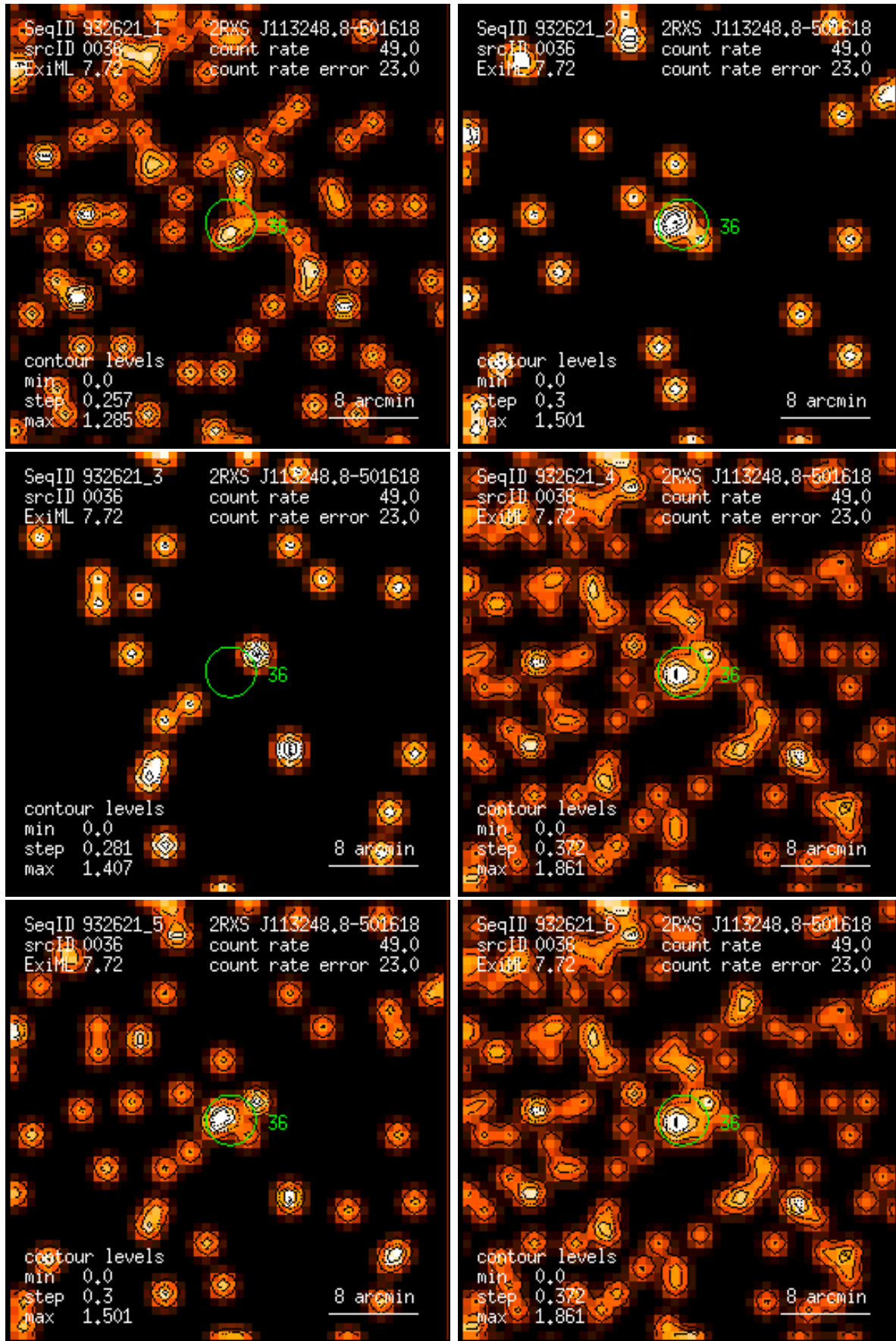
Figure 36: RASS 932621: detection 0036: band rate images, Gaussian filter: (1) PSPC channels 11 – 41, (2) 52 – 90, (3) 91 – 201, (4) 11 – 235, (5) 52 – 201, (6) 11 – 201. Broad band rates in counts/ks. Band rate contour levels in counts/ks/arcmin 2 .
