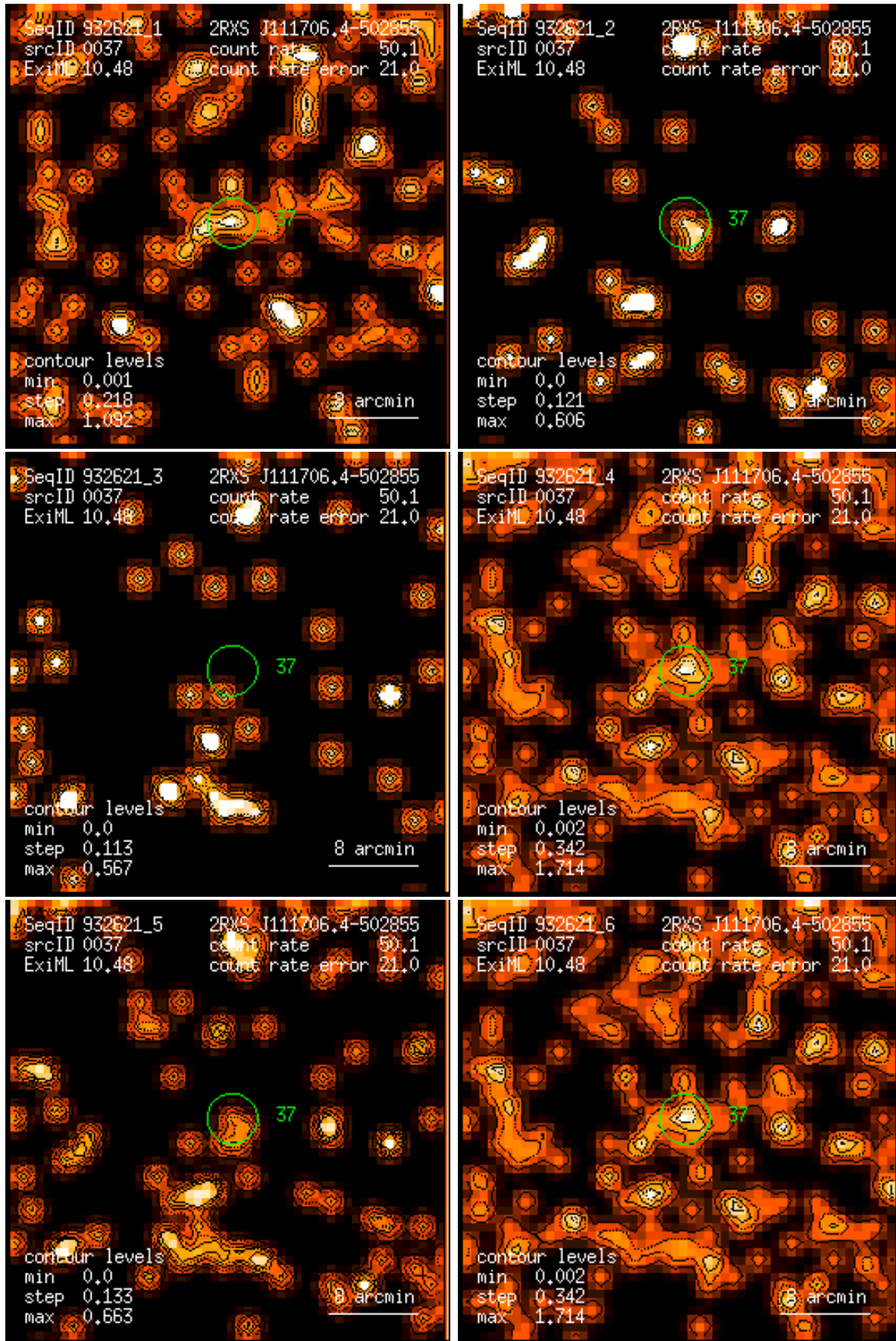
Figure 37: RASS 932621: detection 0037: band rate images, Gaussian filter: (1) PSPC channels 11 – 41, (2) 52 – 90, (3) 91 – 201, (4) 11 – 235, (5) 52 – 201, (6) 11 – 201. Broad band rates in counts/ks. Band rate contour levels in counts/ks/arcmin 2 .
