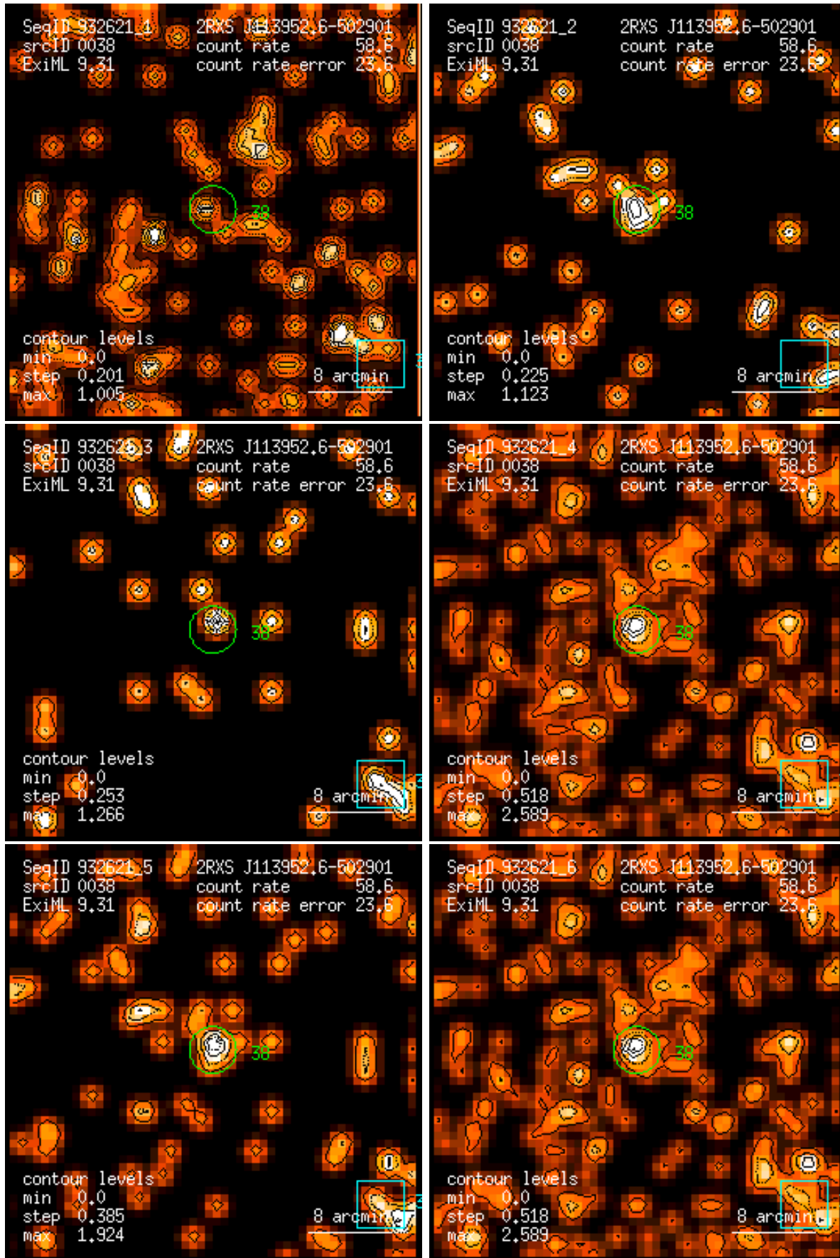
Figure 38: RASS 932621: detection 0038: band rate images, Gaussian filter: (1) PSPC channels 11 – 41, (2) 52 – 90, (3) 91 – 201, (4) 11 – 235, (5) 52 – 201, (6) 11 – 201. Broad band rates in counts/ks. Band rate contour levels in counts/ks/arcmin 2 .
