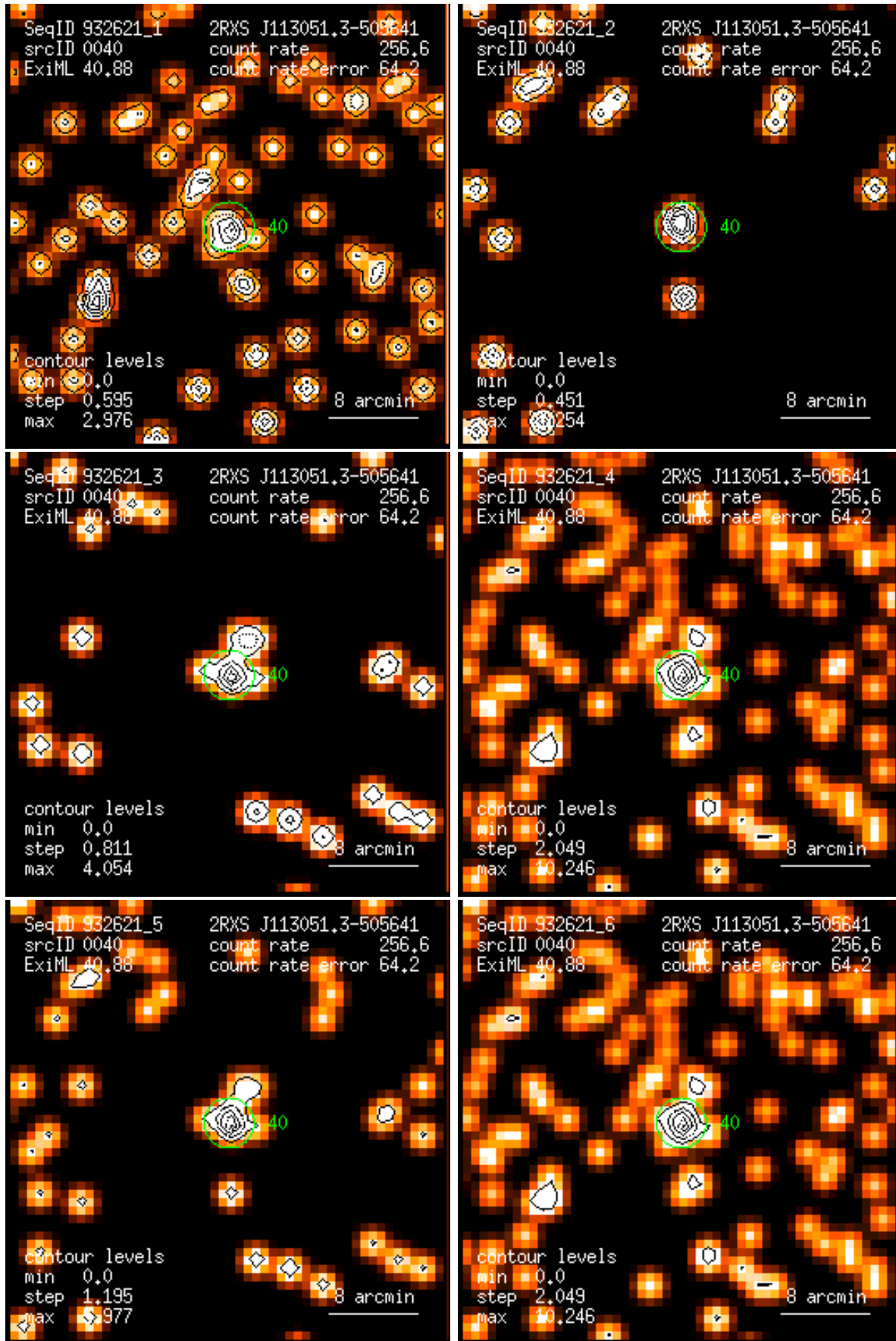
Figure 40: RASS 932621: detection 0040: band rate images, Gaussian filter: (1) PSPC channels 11 – 41, (2) 52 – 90, (3) 91 – 201, (4) 11 – 235, (5) 52 – 201, (6) 11 – 201. Broad band rates in counts/ks. Band rate contour levels in counts/ks/arcmin 2 .
