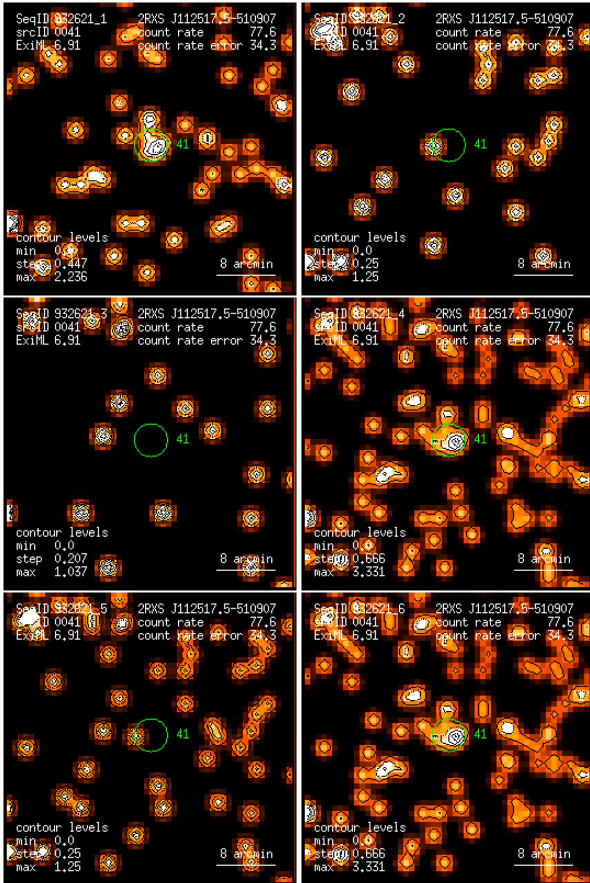
Figure 41: RASS 932621: detection 0041: band rate images, Gaussian filter: (1) PSPC channels 11 – 41, (2) 52 – 90, (3) 91 – 201, (4) 11 – 235, (5) 52 – 201, (6) 11 – 201. Broad band rates in counts/ks. Band rate contour levels in counts/ks/arcmin 2 .
