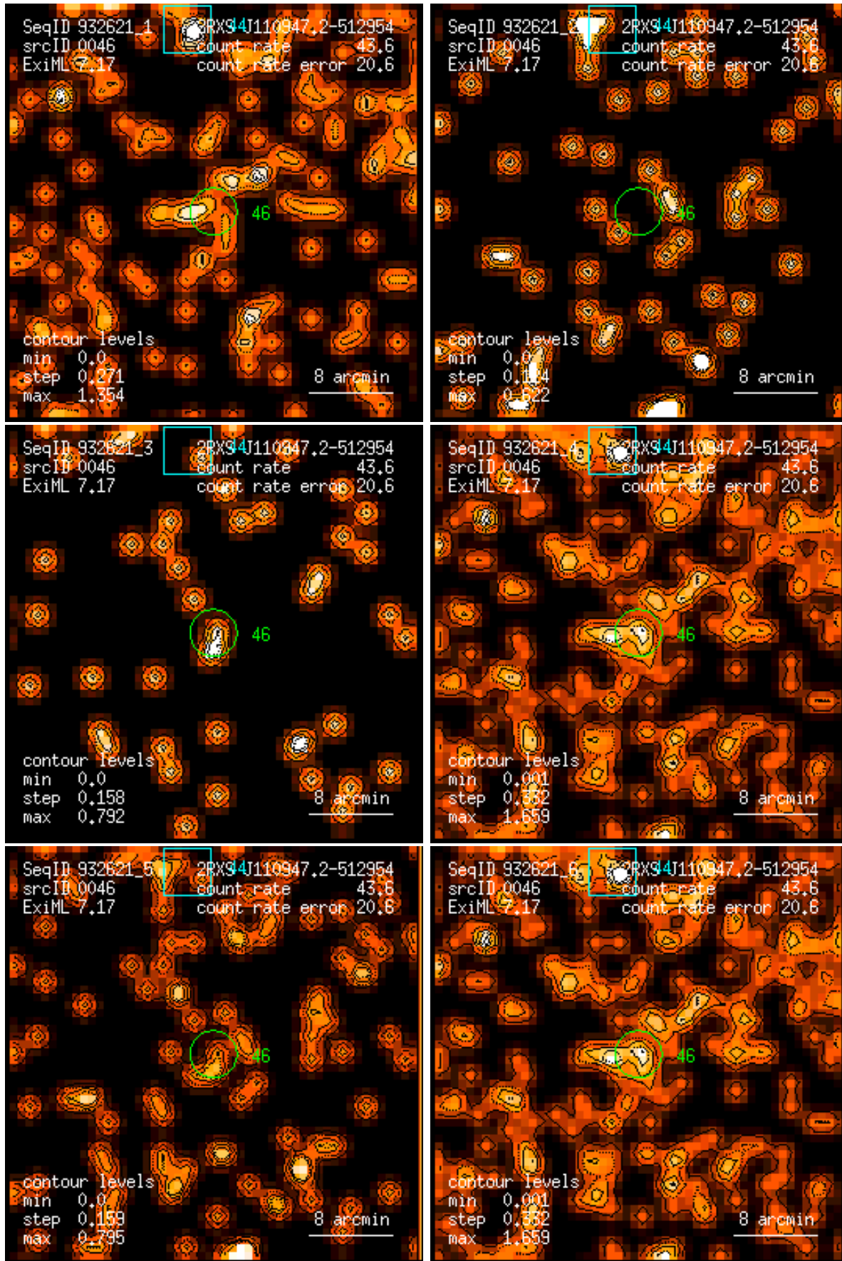
Figure 46: RASS 932621: detection 0046: band rate images, Gaussian filter: (1) PSPC channels 11 – 41, (2) 52 – 90, (3) 91 – 201, (4) 11 – 235, (5) 52 – 201, (6) 11 – 201. Broad band rates in counts/ks. Band rate contour levels in counts/ks/arcmin 2 .
