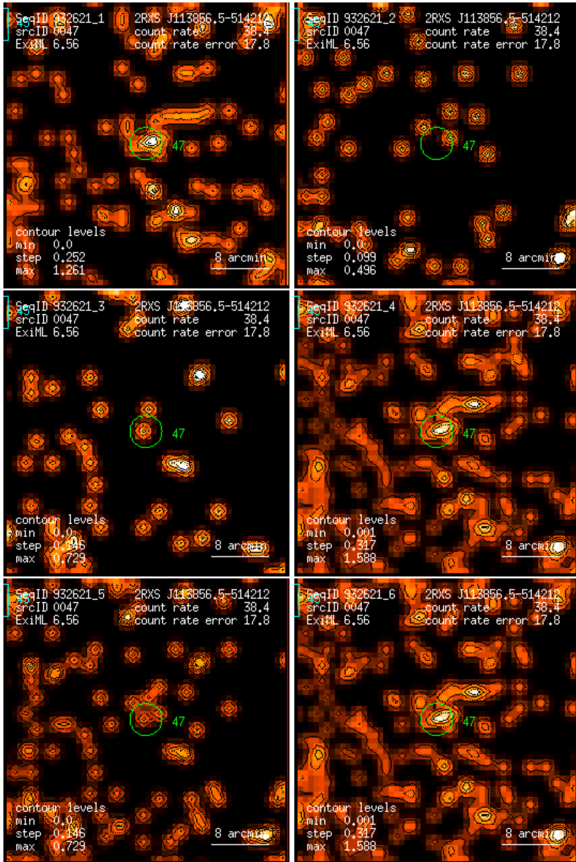
Figure 47: RASS 932621: detection 0047: band rate images, Gaussian filter: (1) PSPC channels 11 – 41, (2) 52 – 90, (3) 91 – 201, (4) 11 – 235, (5) 52 – 201, (6) 11 – 201. Broad band rates in counts/ks. Band rate contour levels in counts/ks/arcmin 2 .
