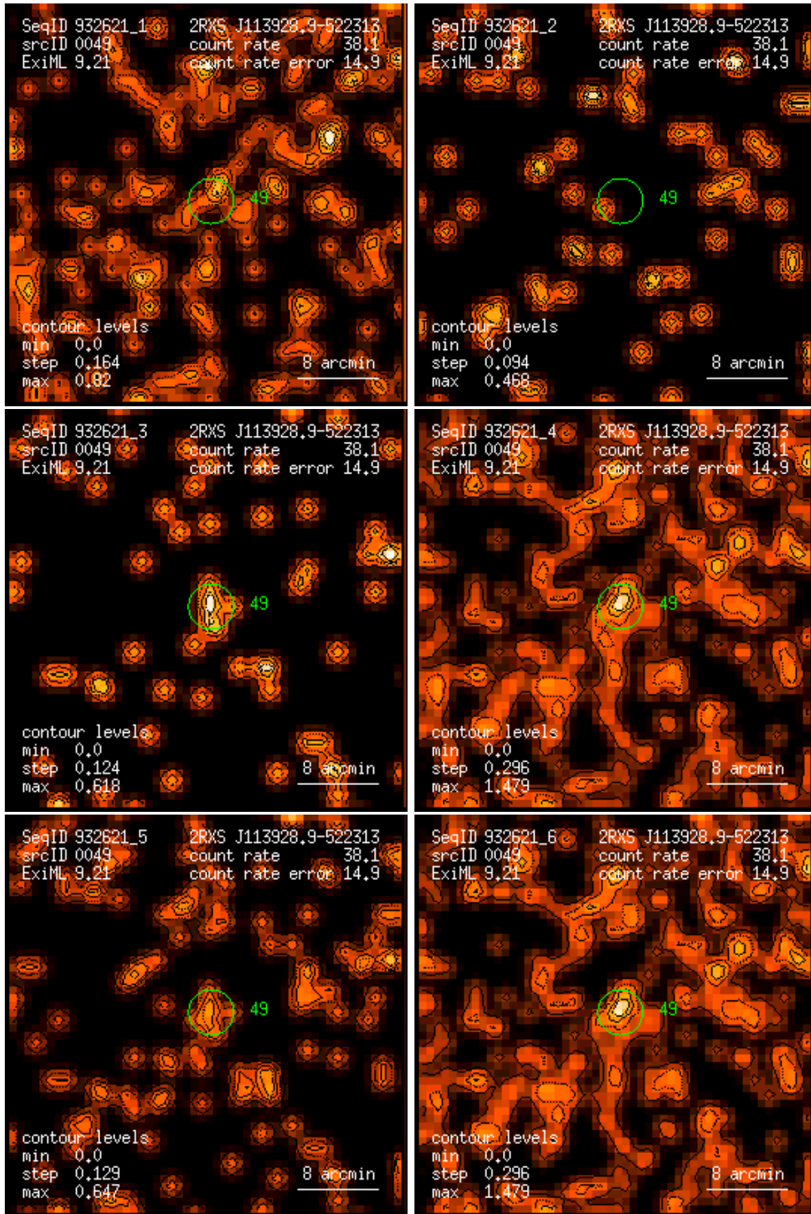
Figure 49: RASS 932621: detection 0049: band rate images, Gaussian filter: (1) PSPC channels 11 – 41, (2) 52 – 90, (3) 91 – 201, (4) 11 – 235, (5) 52 – 201, (6) 11 – 201. Broad band rates in counts/ks. Band rate contour levels in counts/ks/arcmin 2 .
