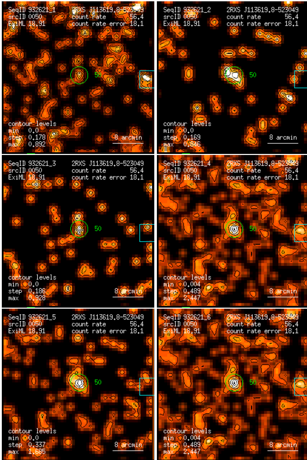
Figure 50: RASS 932621: detection 0050: band rate images, Gaussian filter: (1) PSPC channels 11 – 41, (2) 52 – 90, (3) 91 – 201, (4) 11 – 235, (5) 52 – 201, (6) 11 – 201. Broad band rates in counts/ks. Band rate contour levels in counts/ks/arcmin 2 .
