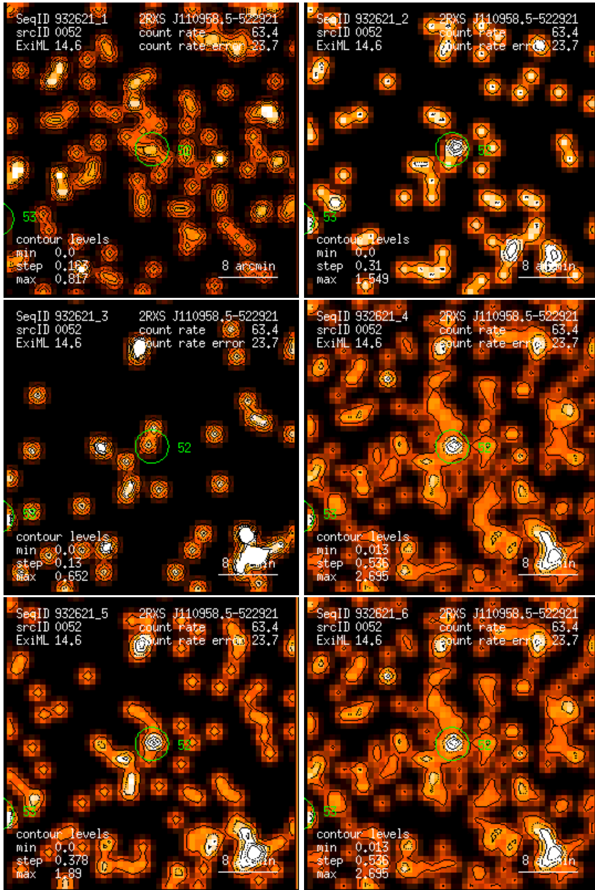
Figure 52: RASS 932621: detection 0052: band rate images, Gaussian filter: (1) PSPC channels 11 – 41, (2) 52 – 90, (3) 91 – 201, (4) 11 – 235, (5) 52 – 201, (6) 11 – 201. Broad band rates in counts/ks. Band rate contour levels in counts/ks/arcmin 2 .
