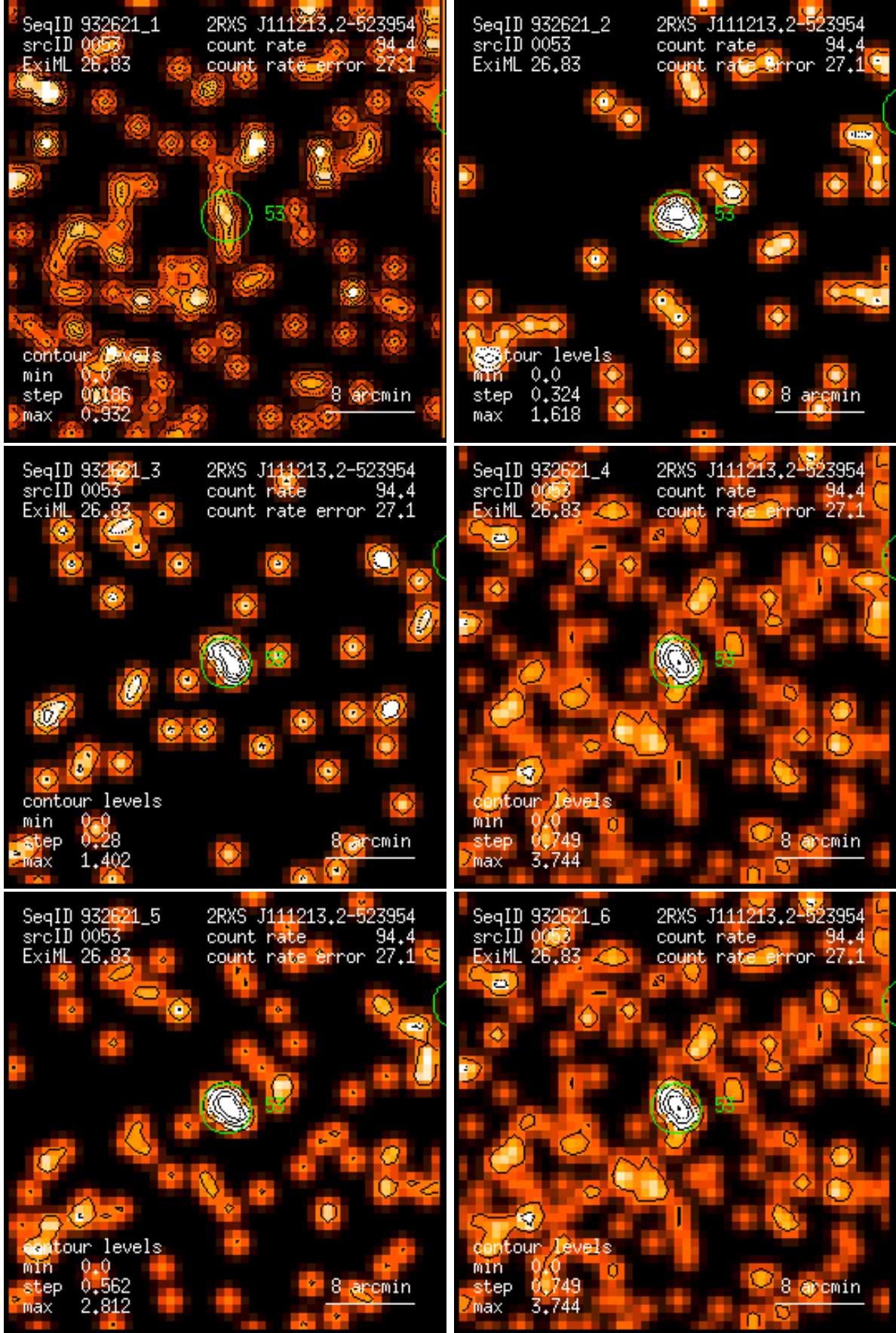
Figure 53: RASS 932621: detection 0053: band rate images, Gaussian filter: (1) PSPC channels 11 – 41, (2) 52 – 90, (3) 91 – 201, (4) 11 – 235, (5) 52 – 201, (6) 11 – 201. Broad band rates in counts/ks. Band rate contour levels in counts/ks/arcmin 2 .
