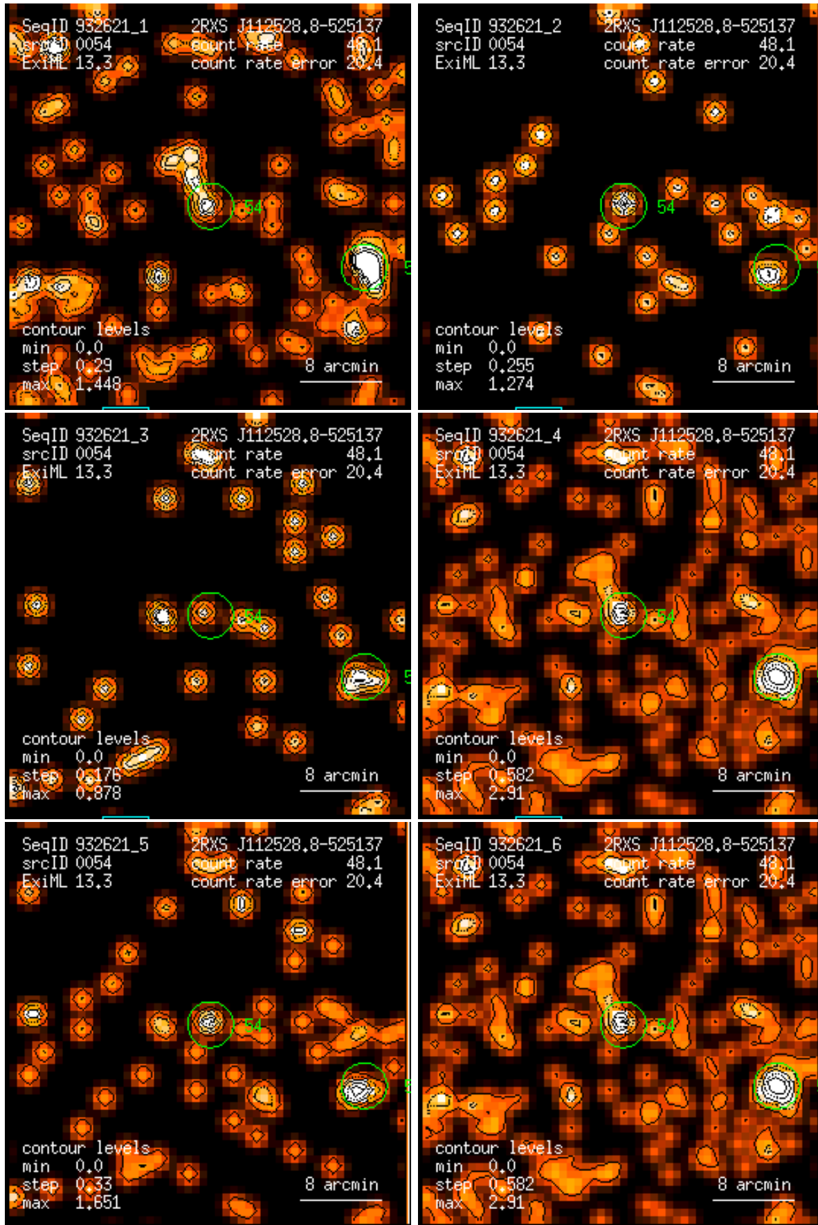
Figure 54: RASS 932621: detection 0054: band rate images, Gaussian filter: (1) PSPC channels 11 – 41, (2) 52 – 90, (3) 91 – 201, (4) 11 – 235, (5) 52 – 201, (6) 11 – 201. Broad band rates in counts/ks. Band rate contour levels in counts/ks/arcmin 2 .
