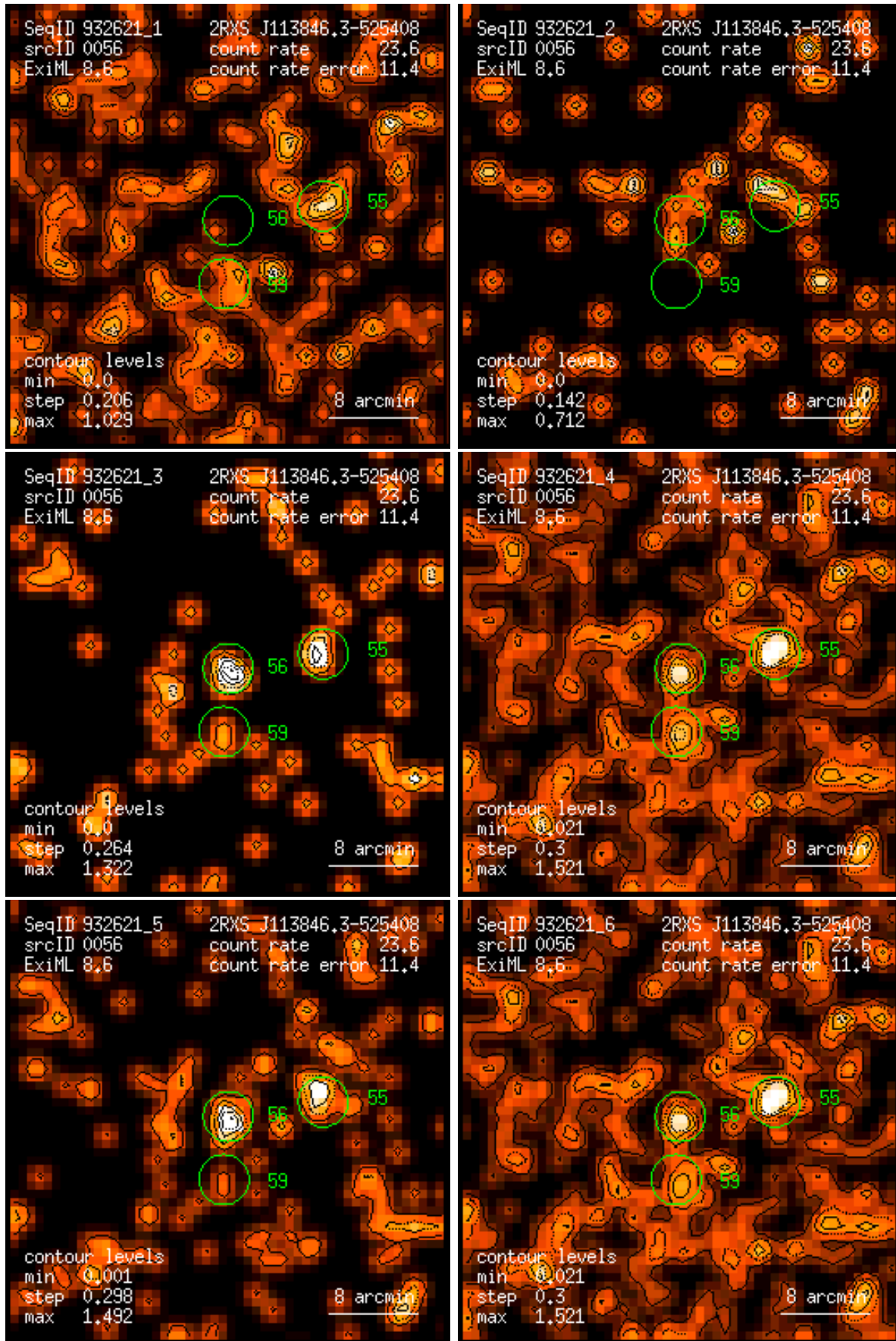
Figure 56: RASS 932621: detection 0056: band rate images, Gaussian filter: (1) PSPC channels 11 – 41, (2) 52 – 90, (3) 91 – 201, (4) 11 – 235, (5) 52 – 201, (6) 11 – 201. Broad band rates in counts/ks. Band rate contour levels in counts/ks/arcmin 2 .
