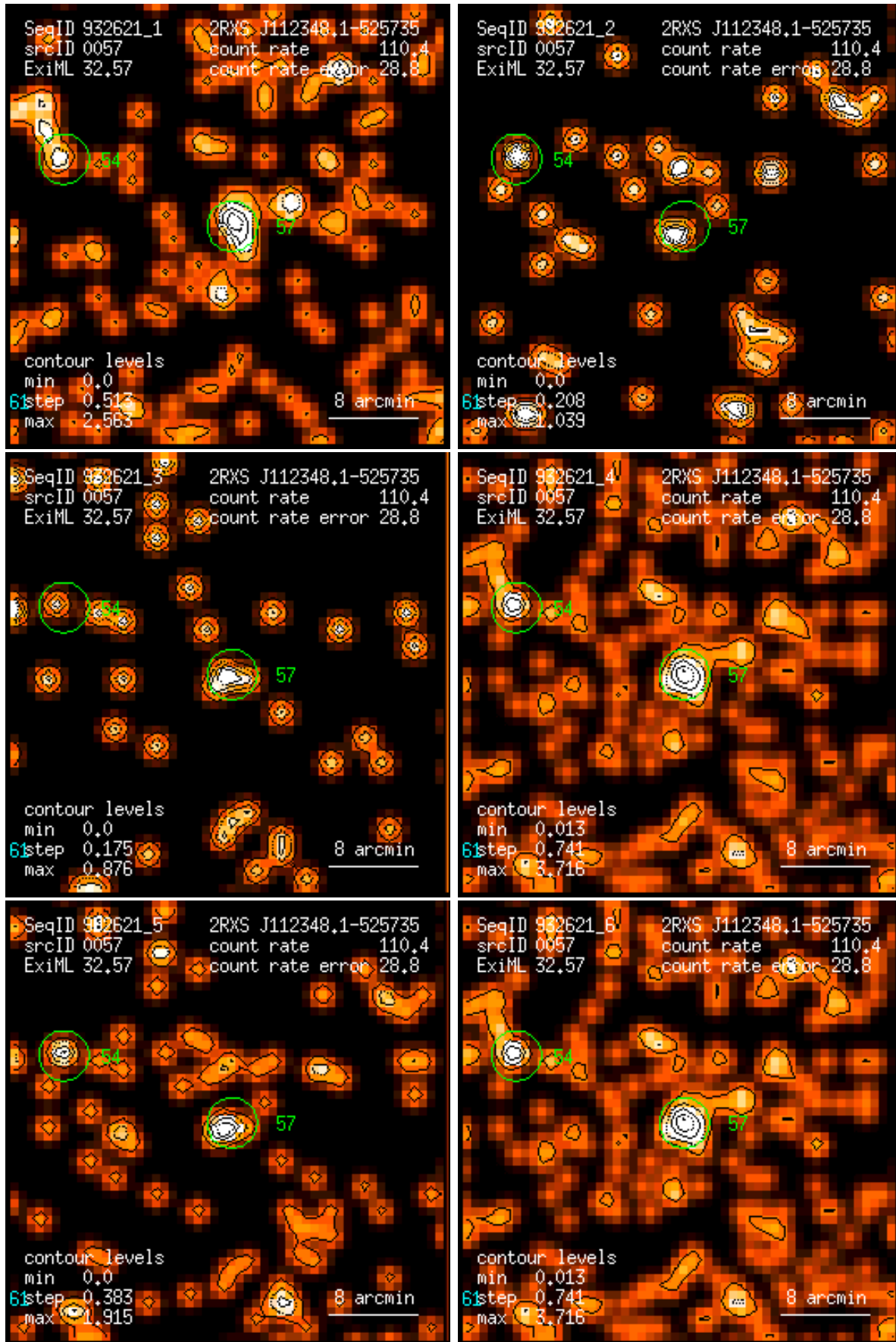
Figure 57: RASS 932621: detection 0057: band rate images, Gaussian filter: (1) PSPC channels 11 – 41, (2) 52 – 90, (3) 91 – 201, (4) 11 – 235, (5) 52 – 201, (6) 11 – 201. Broad band rates in counts/ks. Band rate contour levels in counts/ks/arcmin 2 .
