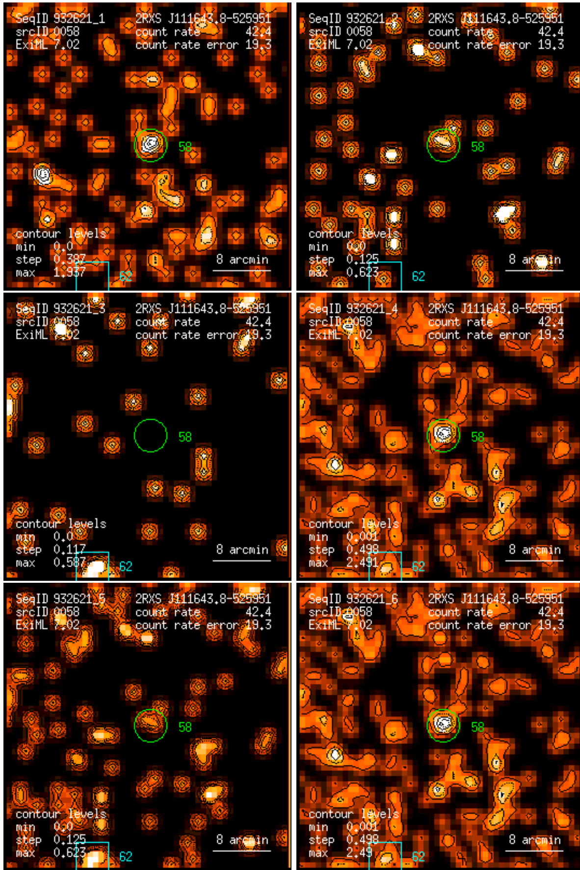
Figure 58: RASS 932621: detection 0058: band rate images, Gaussian filter: (1) PSPC channels 11 – 41, (2) 52 – 90, (3) 91 – 201, (4) 11 – 235, (5) 52 – 201, (6) 11 – 201. Broad band rates in counts/ks. Band rate contour levels in counts/ks/arcmin 2 .
