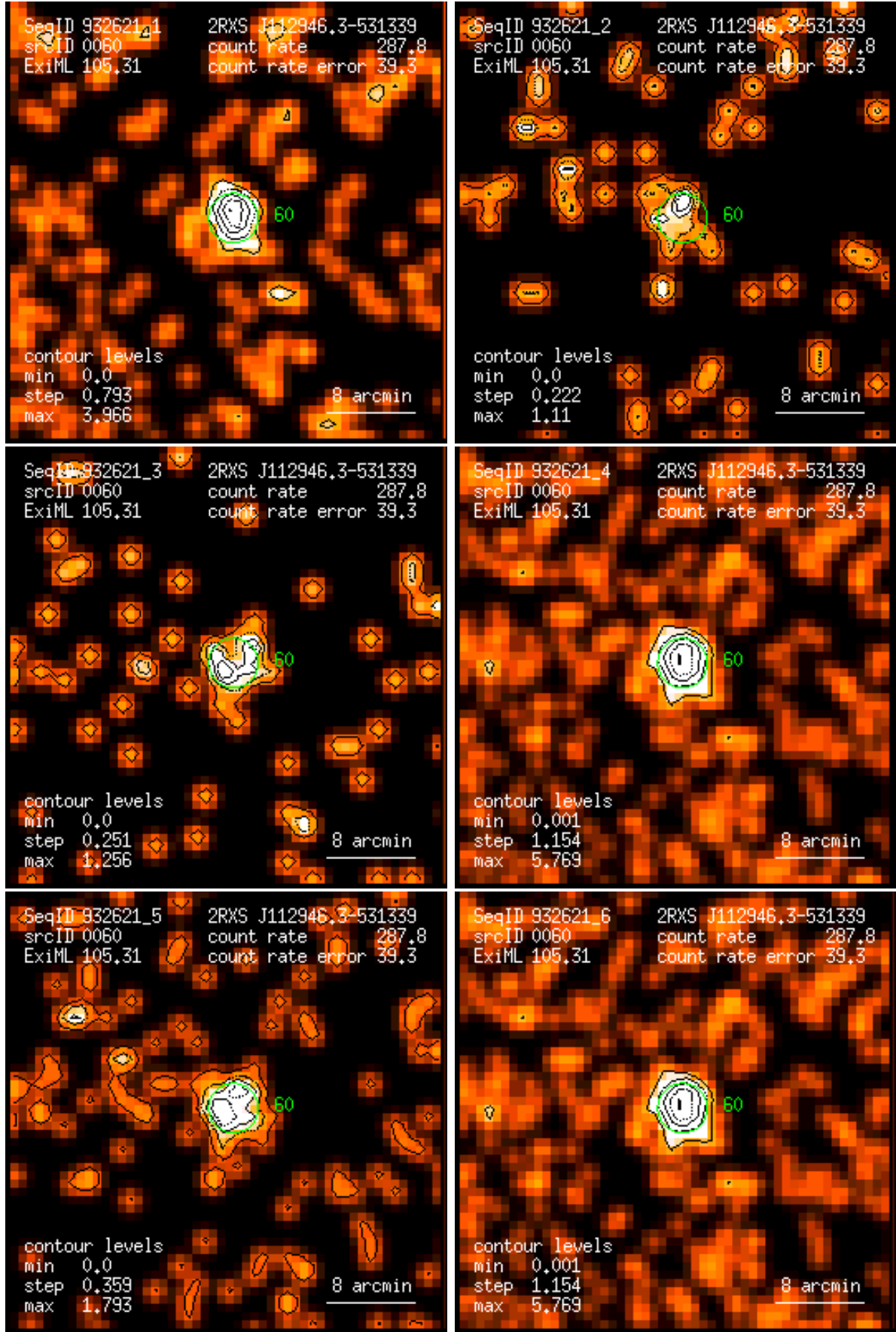
Figure 60: RASS 932621: detection 0060: band rate images, Gaussian filter: (1) PSPC channels 11 – 41, (2) 52 – 90, (3) 91 – 201, (4) 11 – 235, (5) 52 – 201, (6) 11 – 201. Broad band rates in counts/ks. Band rate contour levels in counts/ks/arcmin 2 .
