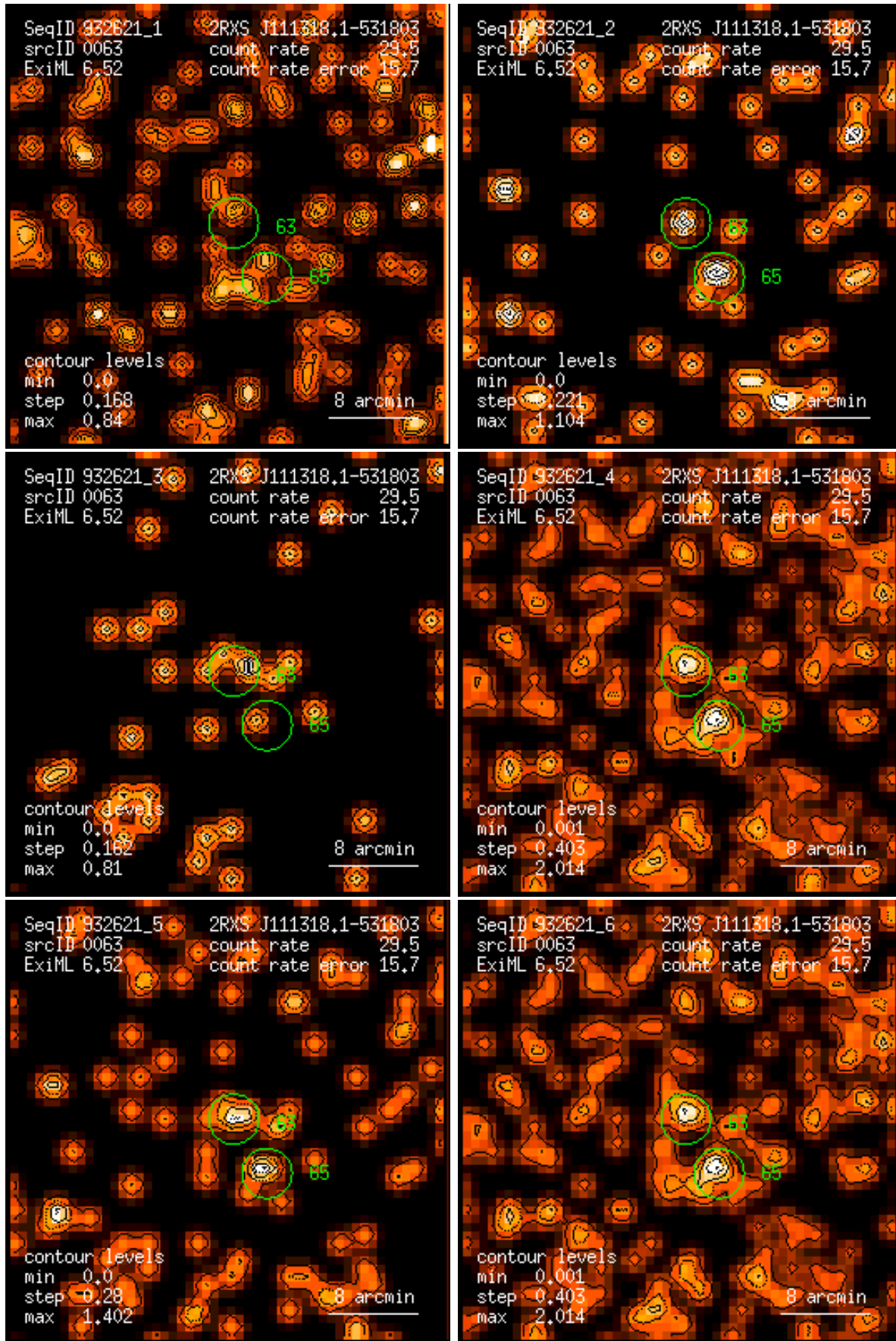
Figure 63: RASS 932621: detection 0063: band rate images, Gaussian filter: (1) PSPC channels 11 – 41, (2) 52 – 90, (3) 91 – 201, (4) 11 – 235, (5) 52 – 201, (6) 11 – 201. Broad band rates in counts/ks. Band rate contour levels in counts/ks/arcmin 2 .
