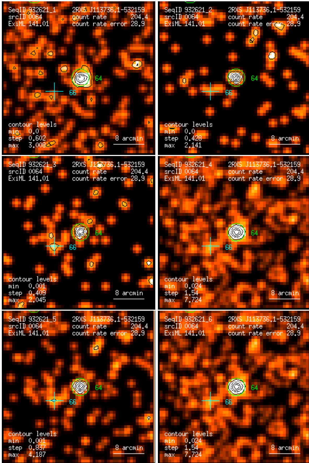
Figure 64: RASS 932621: detection 0064: band rate images, Gaussian filter: (1) PSPC channels 11 – 41, (2) 52 – 90, (3) 91 – 201, (4) 11 – 235, (5) 52 – 201, (6) 11 – 201. Broad band rates in counts/ks. Band rate contour levels in counts/ks/arcmin 2 .
