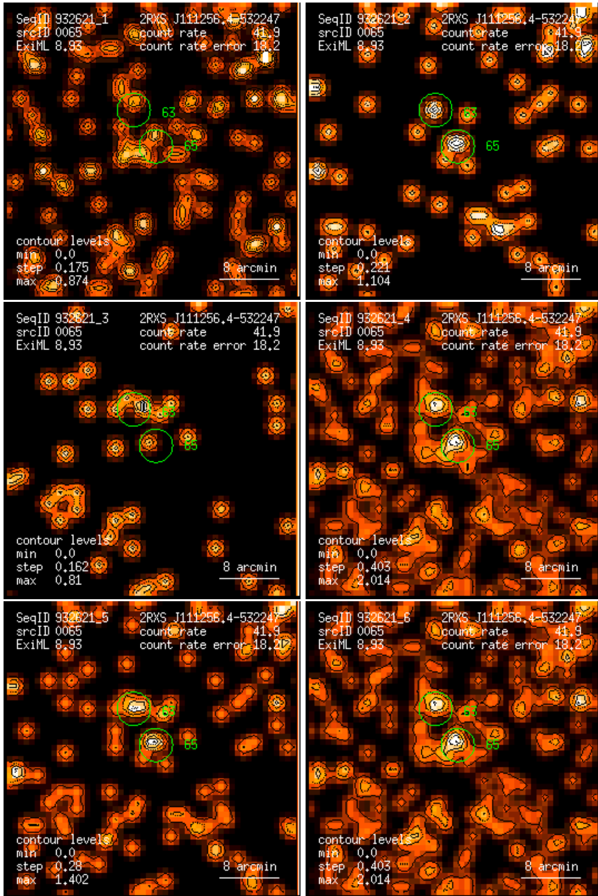
Figure 65: RASS 932621: detection 0065: band rate images, Gaussian filter: (1) PSPC channels 11 – 41, (2) 52 – 90, (3) 91 – 201, (4) 11 – 235, (5) 52 – 201, (6) 11 – 201. Broad band rates in counts/ks. Band rate contour levels in counts/ks/arcmin 2 .
